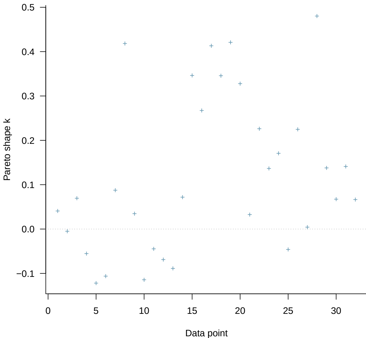
PSIS diagnostic plot
