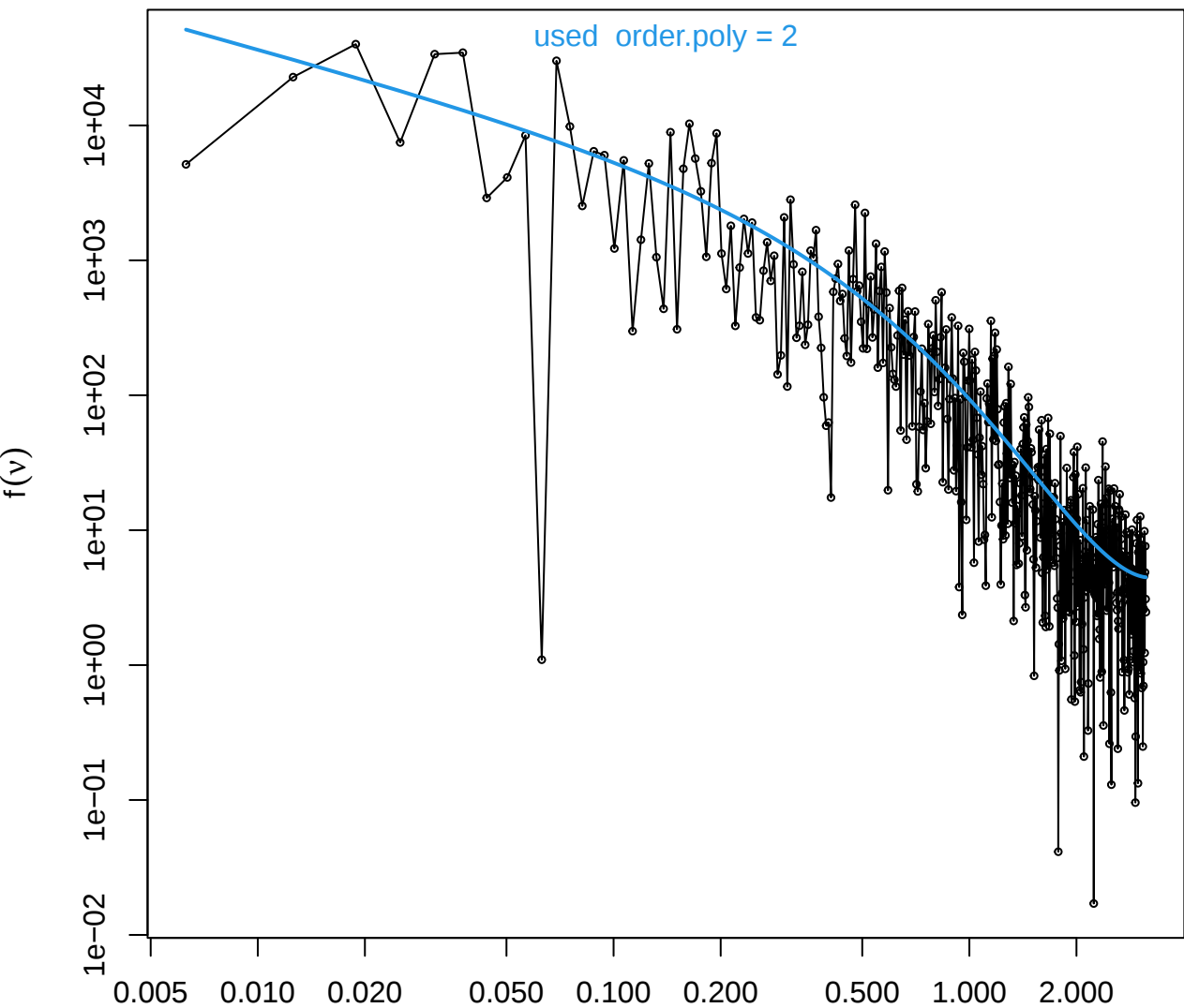
v = 2\pi j/n, j \in 1 \dots 499, n = 1000 Data periodogram and fitted (FEXP) spectrum [log - log]
