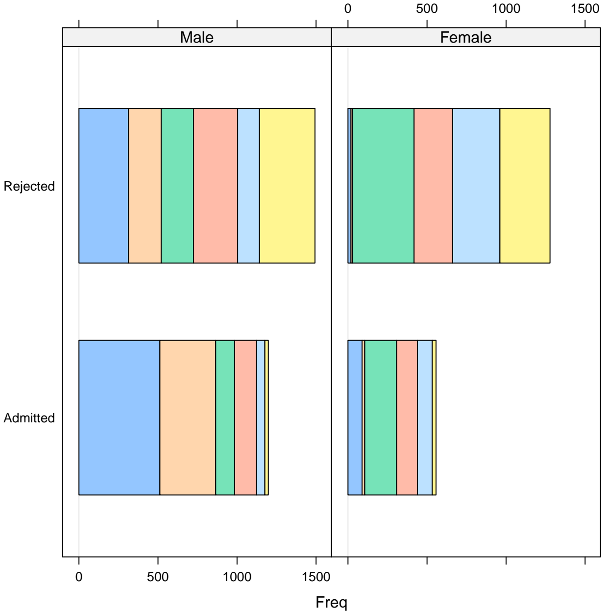
barchart(UCBAdmissions)
