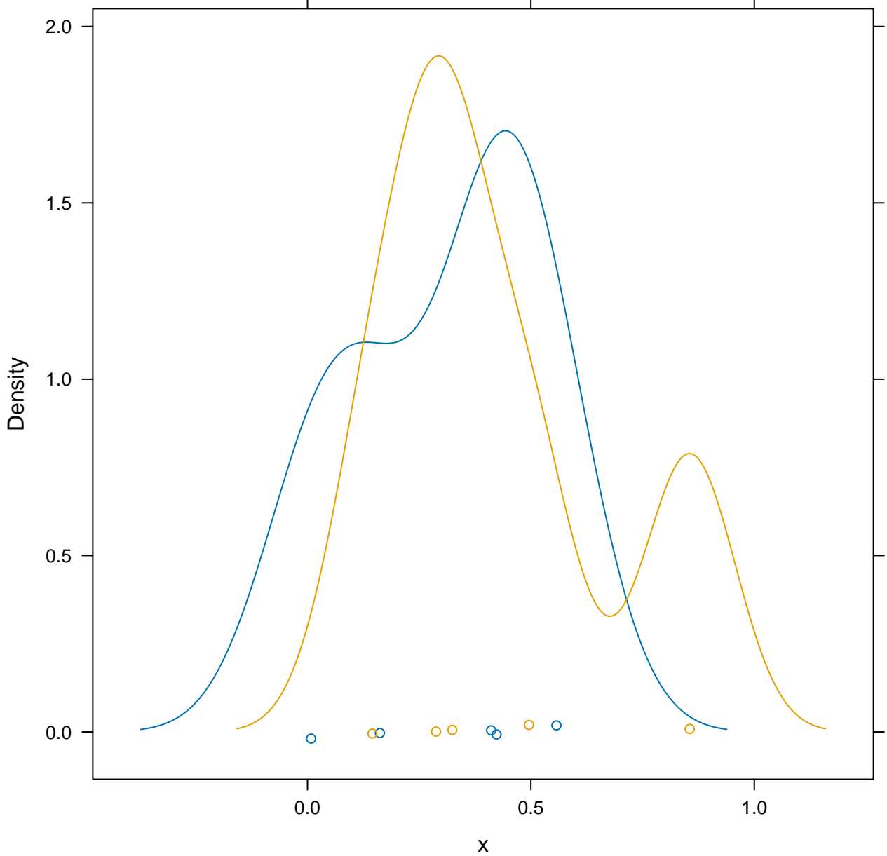
densityplot(~x, groups = g2)
