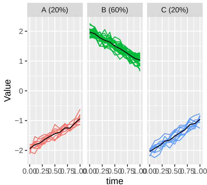
Cluster trajectories
