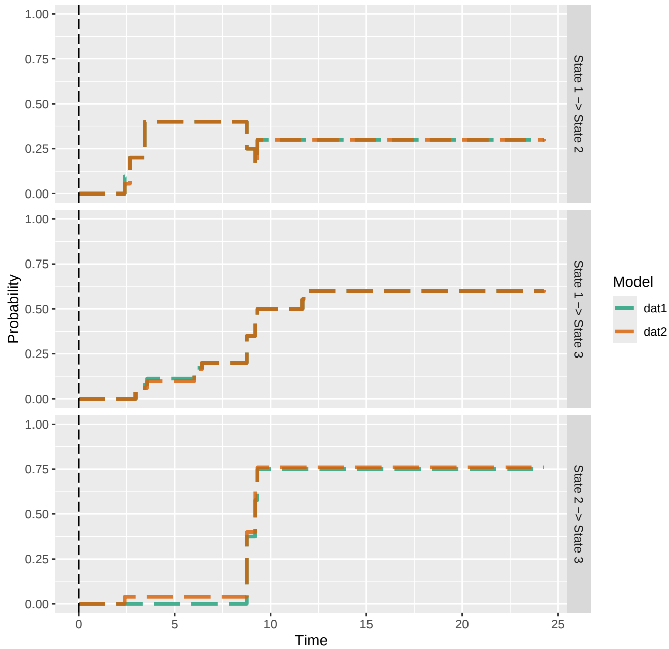
Transition probabilities
