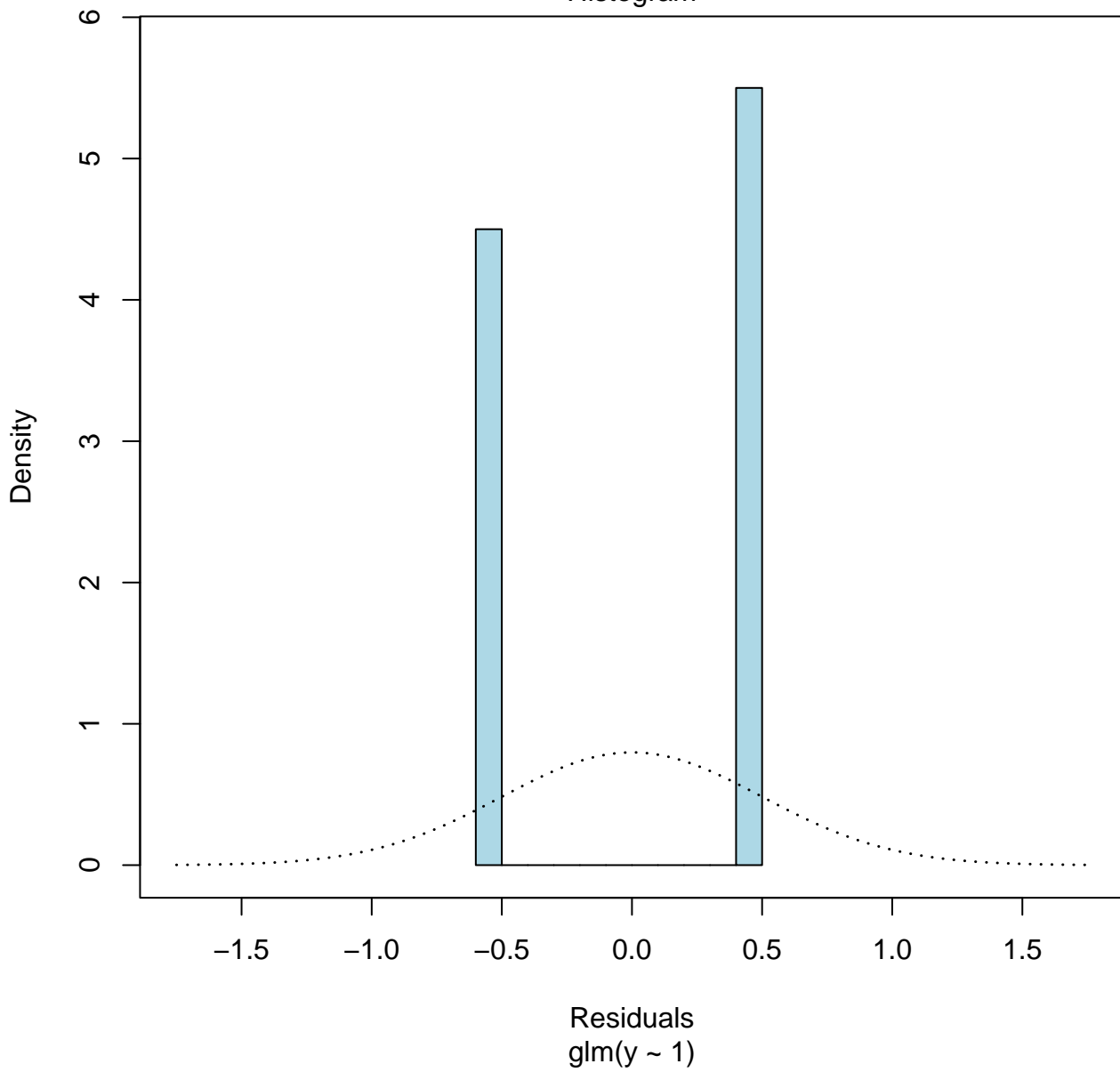
Histogram
