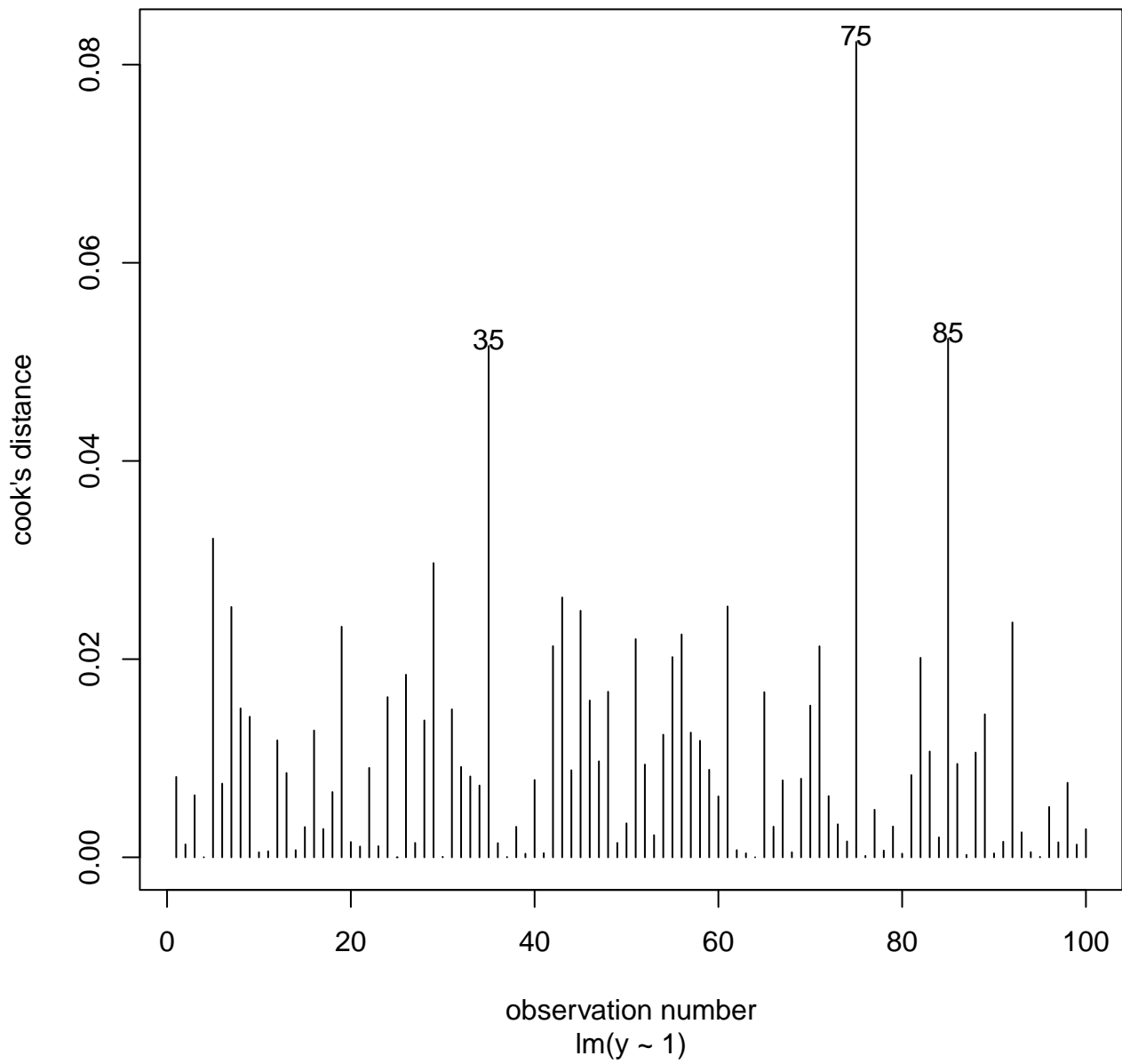
Cook's distance
