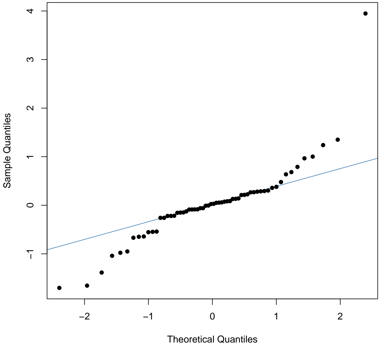
Q-Q plot for Errors (pivoted Cholesky decomposition)
