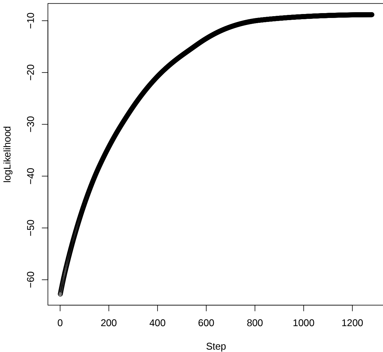
logLik from MCM GMIFS fit
