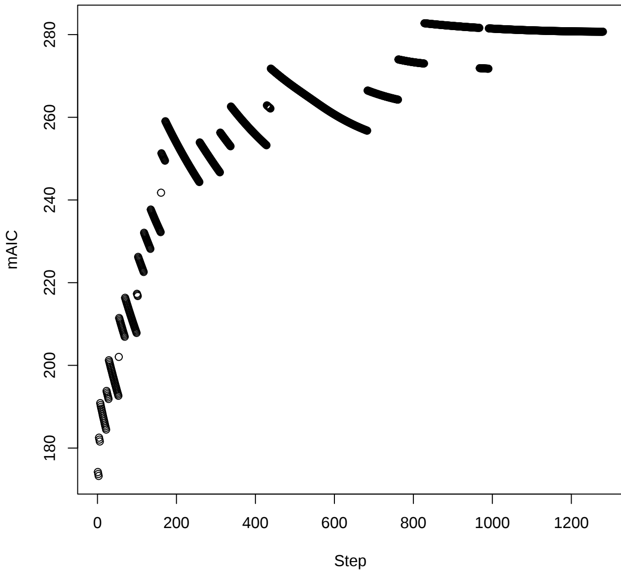
mAIC from MCM GMIFS fit
