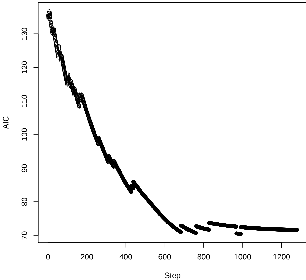
AIC from MCM GMIFS fit
