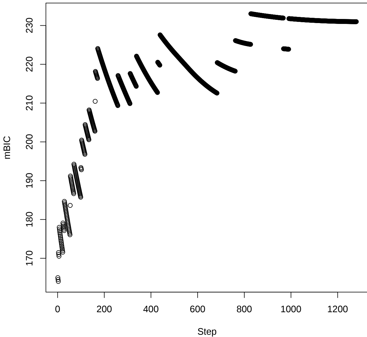
mBIC from MCM GMIFS fit
