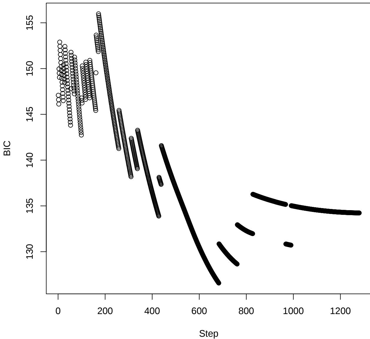
BIC from MCM GMIFS fit
