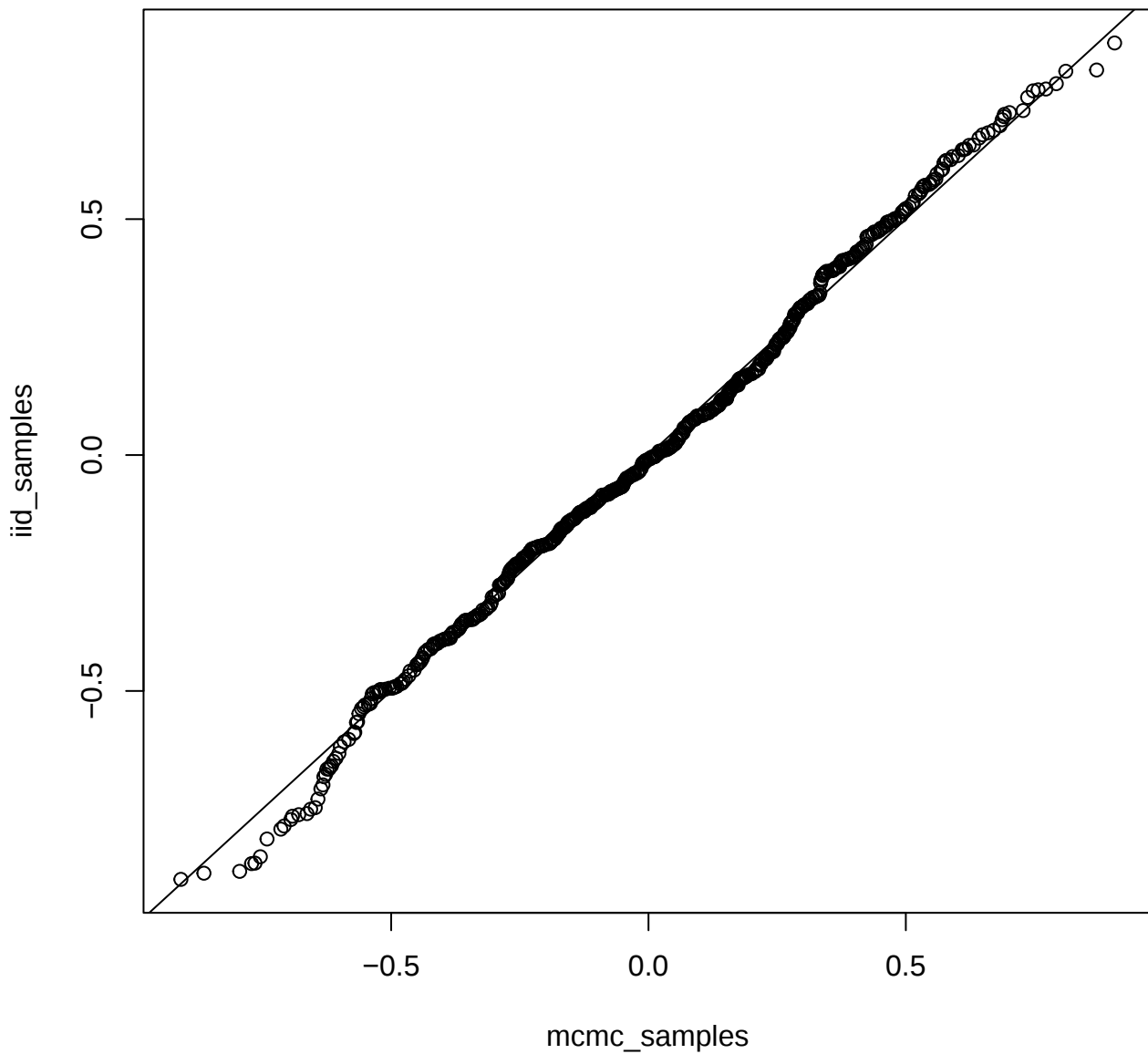
lkj_correlation with hmc sampler
