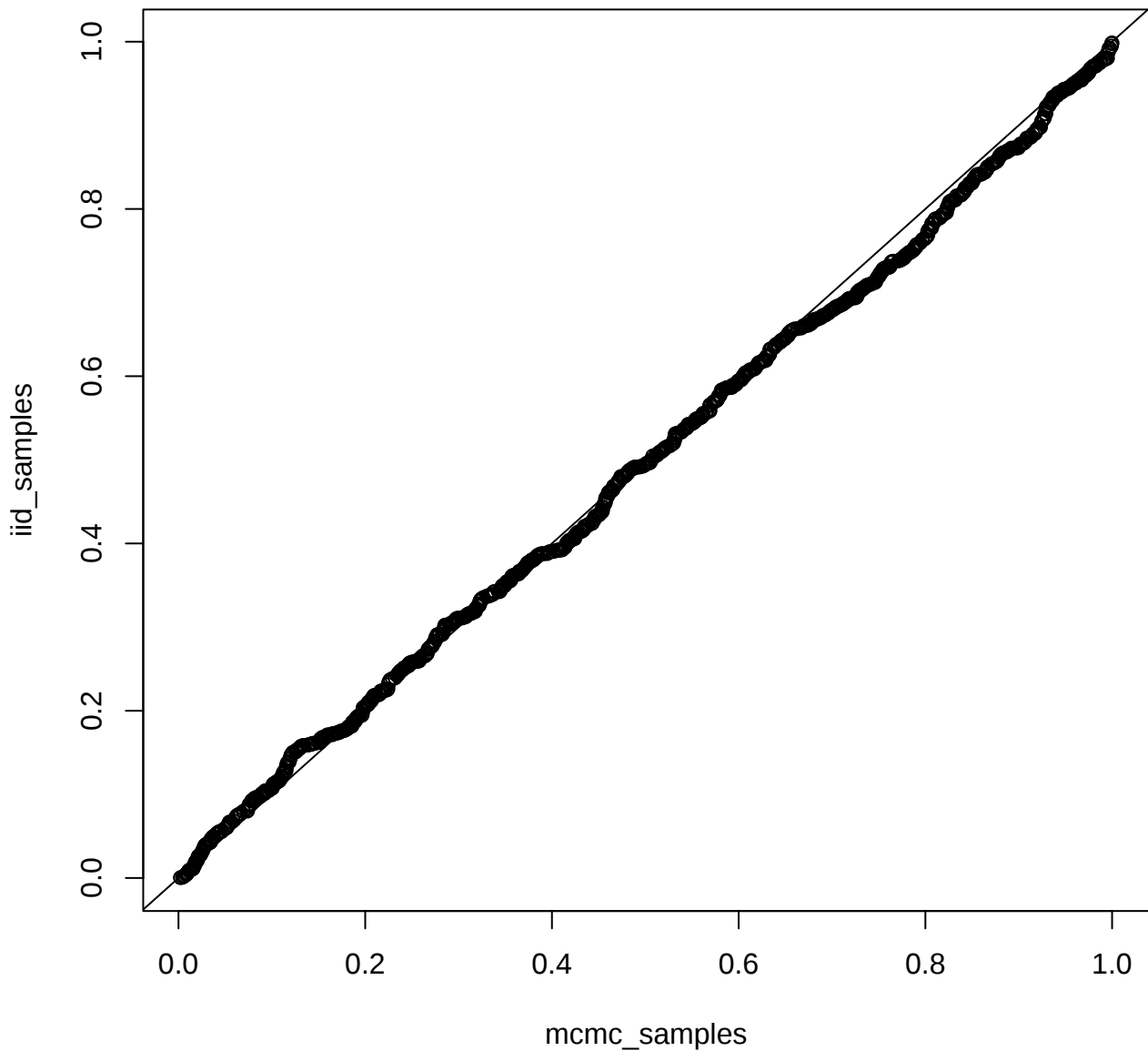
uniform with hmc sampler
