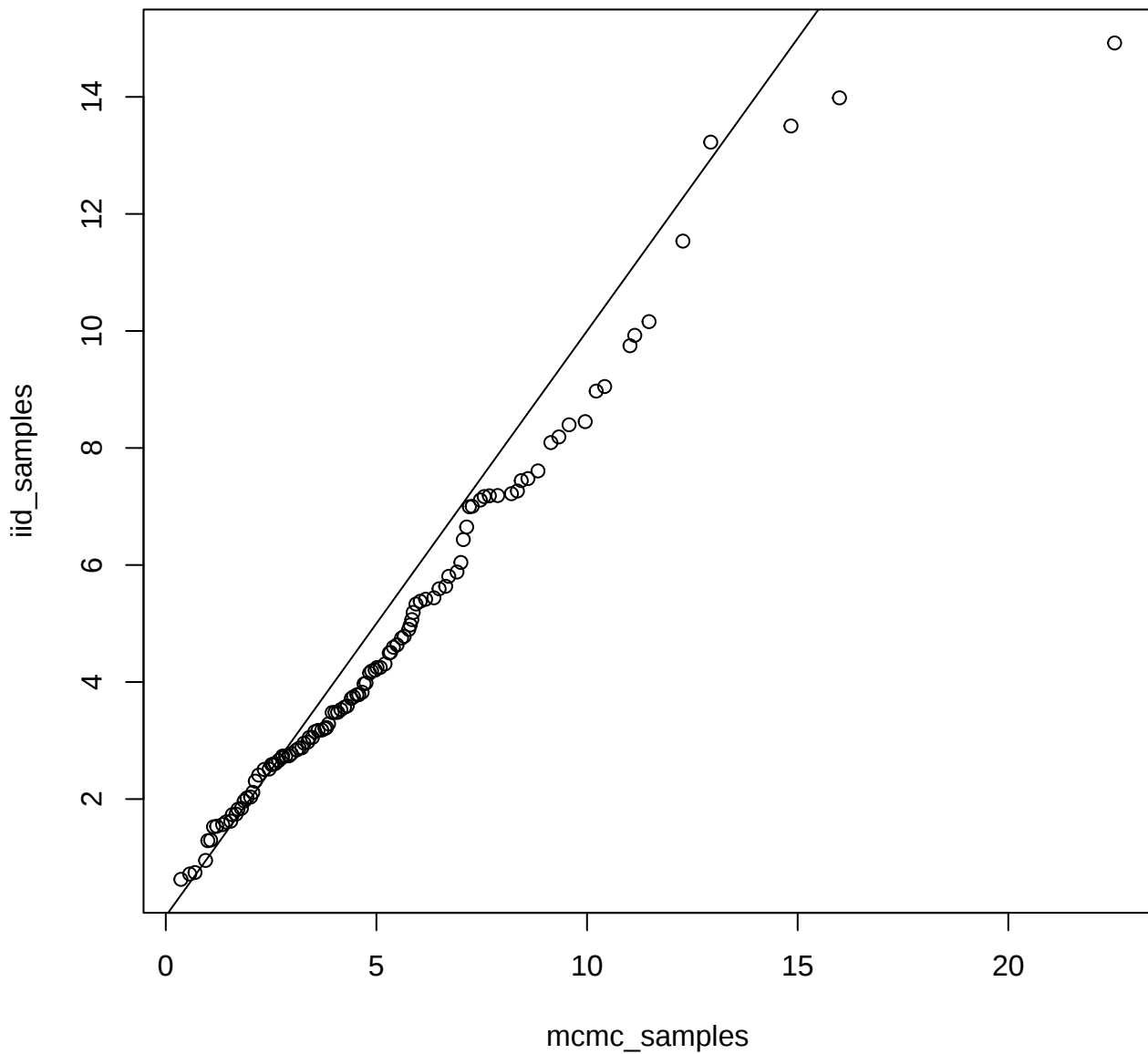
chi_squared with hmc sampler
