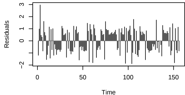
Pearson Residuals
