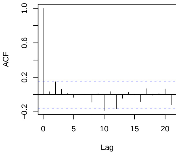
ACF of Randomized Residuals
