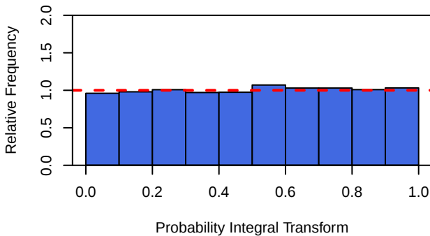
Histogram of Uniform PIT
