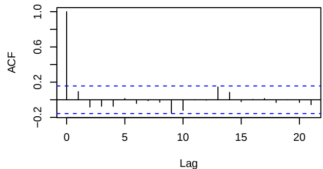
ACF of Randomized Residuals
