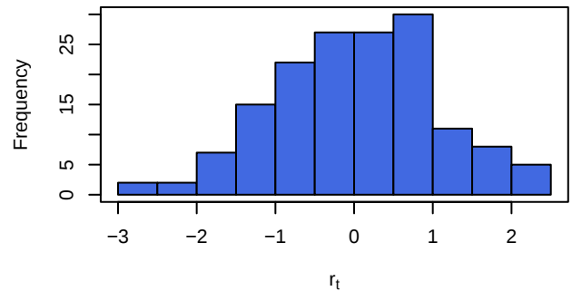
Histogram of Randomized Residuals
