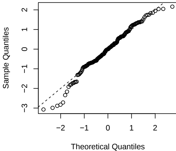
Q-Q Plot of Randomized Residuals
