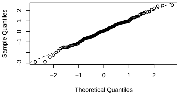
Q-Q Plot of Randomized Residuals
