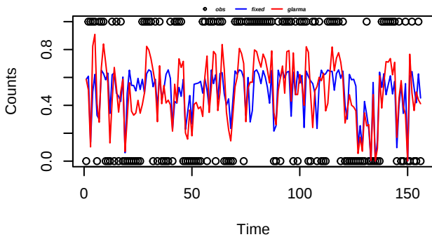
Observed vs Fixed vs GLARMA
