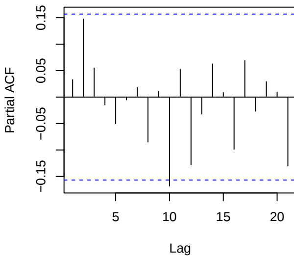
PACF of Randomized Residuals
