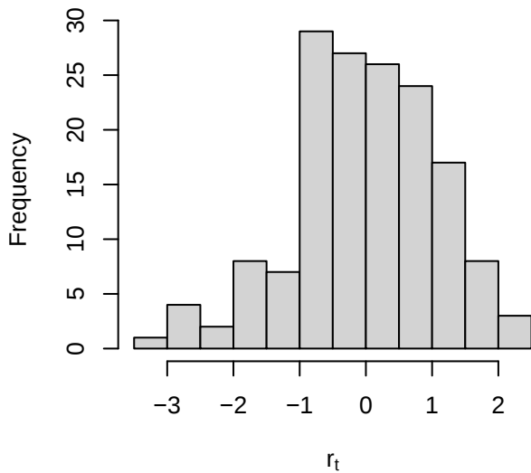
Histogram of Randomized Residuals
