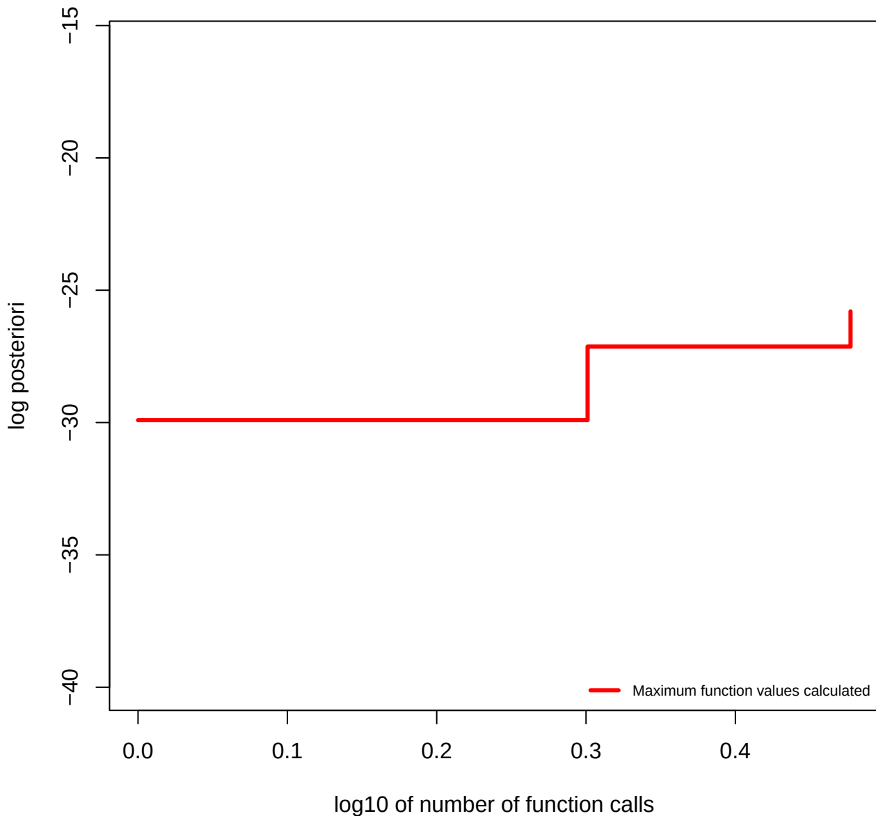
Convergence plot
