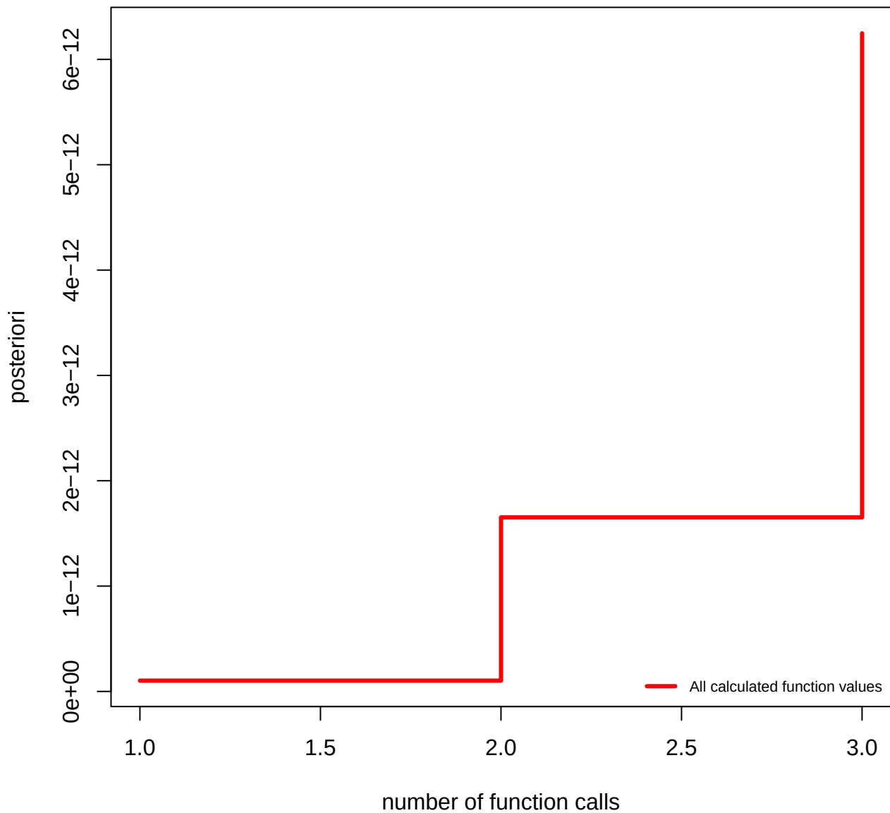
Convergence plot
