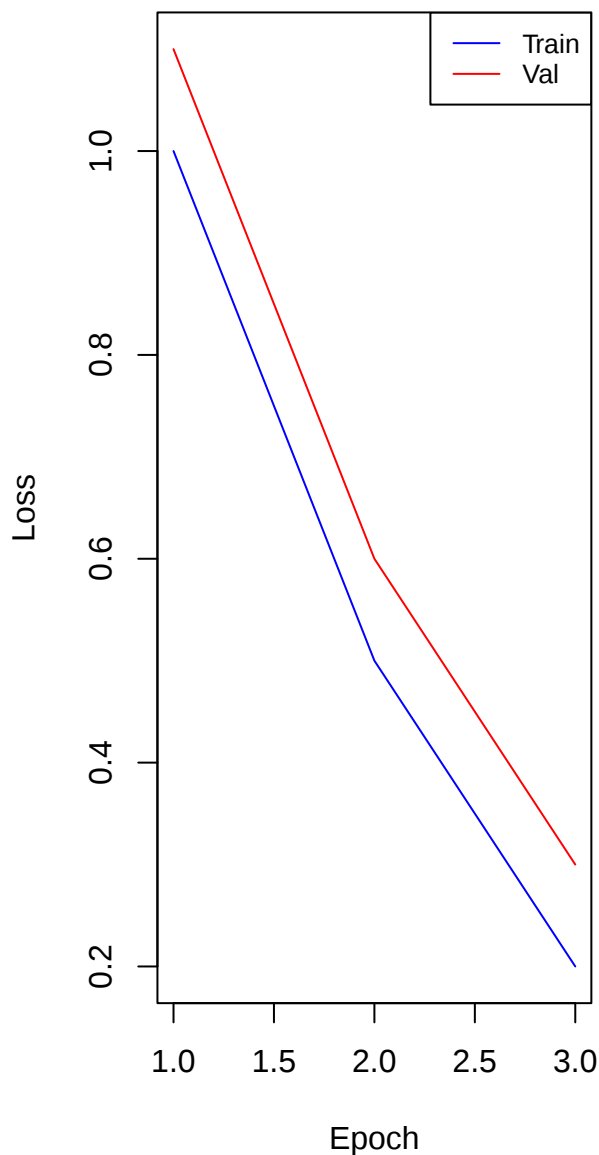
Loss
