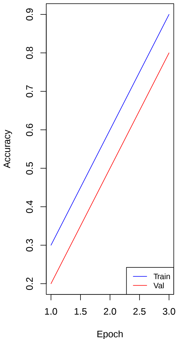
Accuracy
