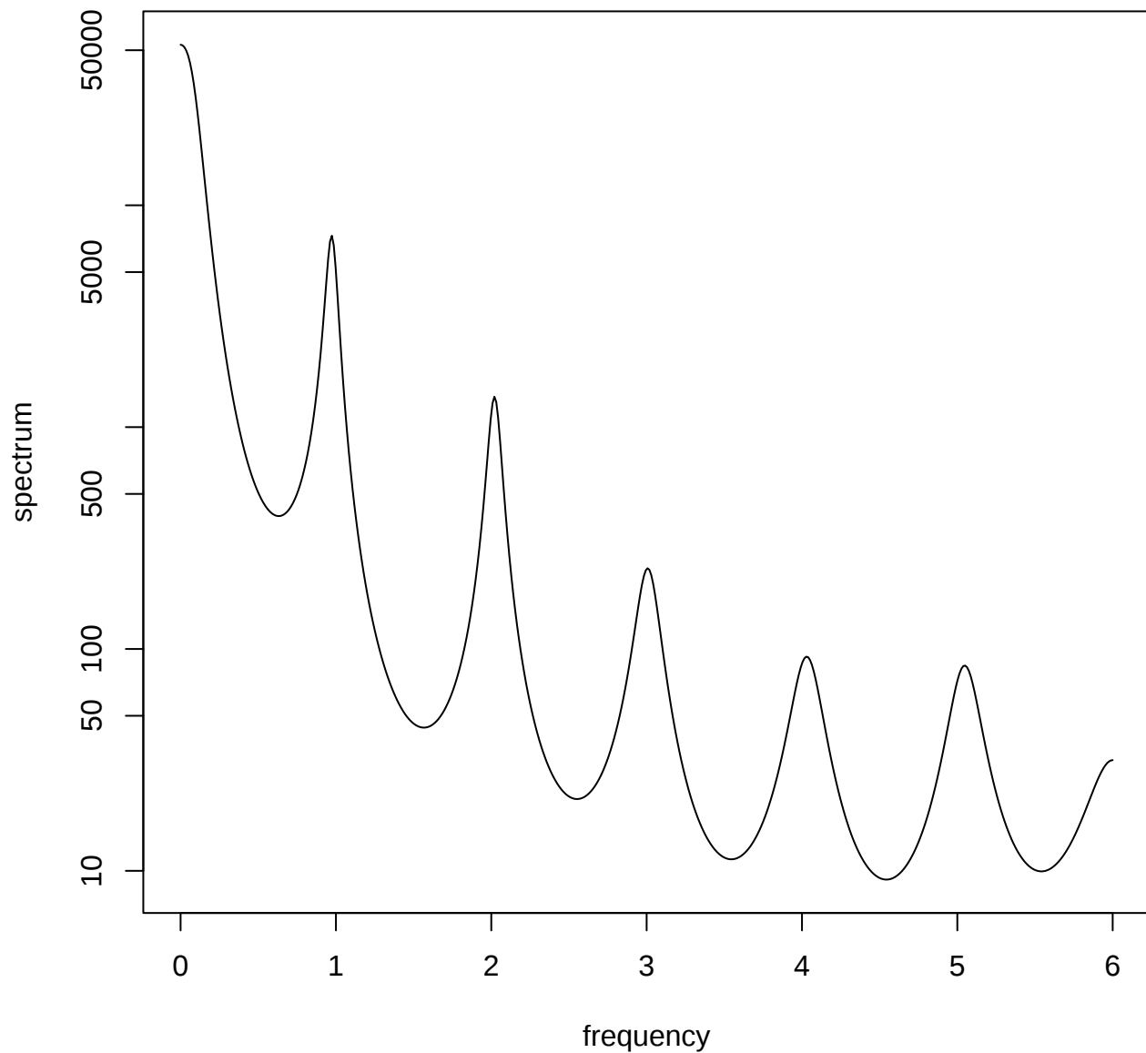
Series: AirPassengers AR (13) spectrum
