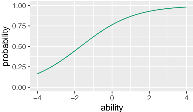
Item Characteristic Curve, Item03
