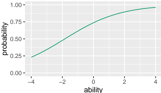
Item Characteristic Curve, Item05
