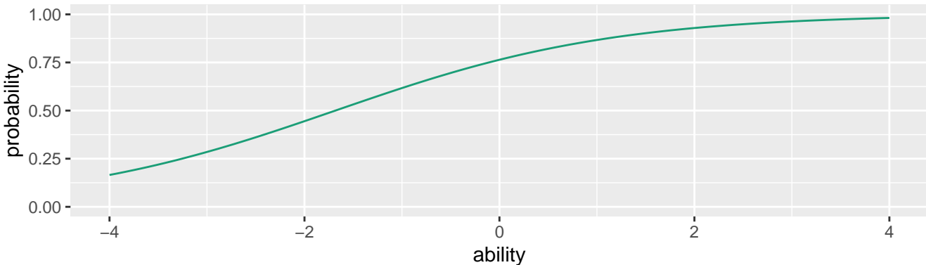
Item Characteristic Curve, Item02
