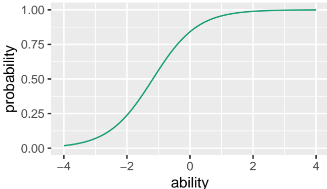
Item Characteristic Curve, Item06
