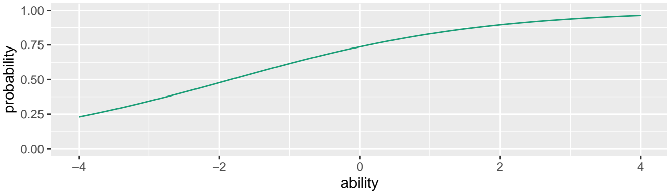
Item Characteristic Curve, Item03
