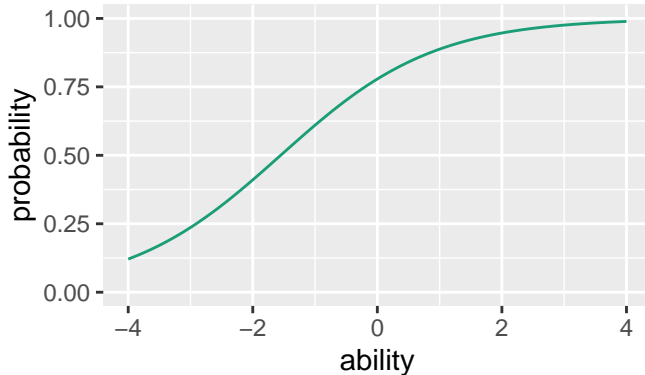
Item Characteristic Curve, Item04
