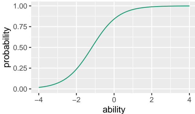
Item Characteristic Curve, Item06
