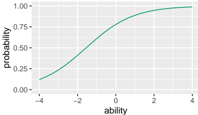
Item Characteristic Curve, Item04
