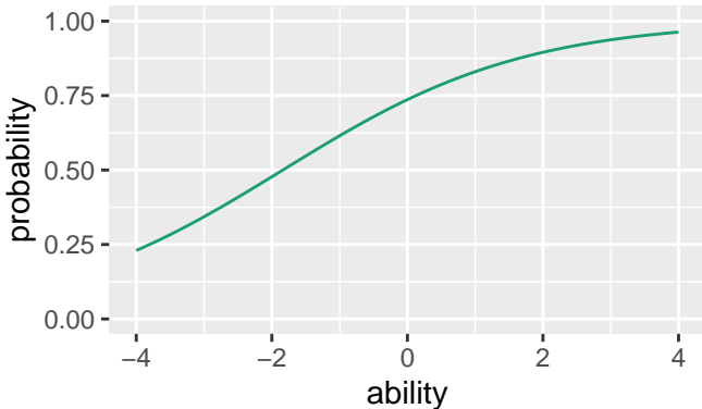
Item Characteristic Curve, Item05
