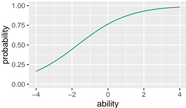
Item Characteristic Curve, Item03
