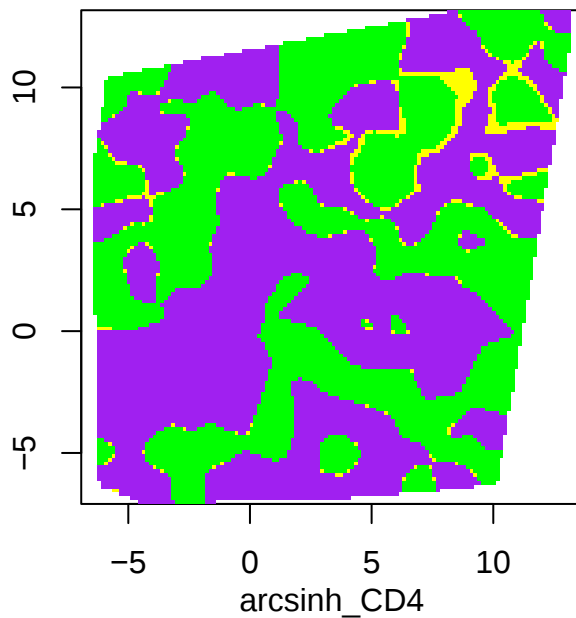
significant p-values ( \alpha = 5.00\text{e-}02 )
