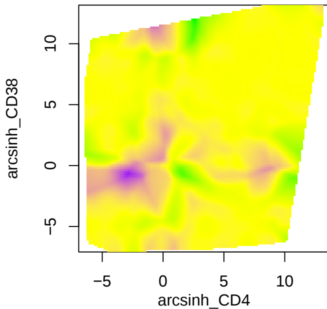
log of the relative risk surfaces (bandwidth: 0.512 units)
