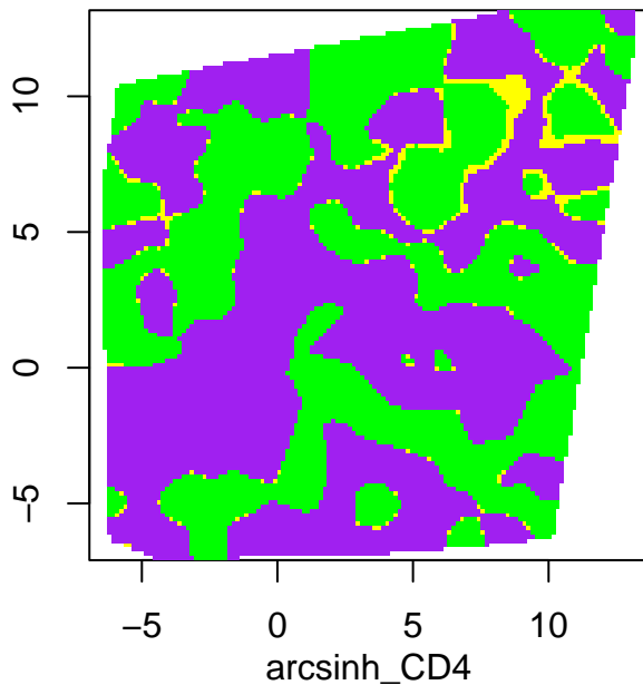
significant p-values (alpha = 5.00e-02)
