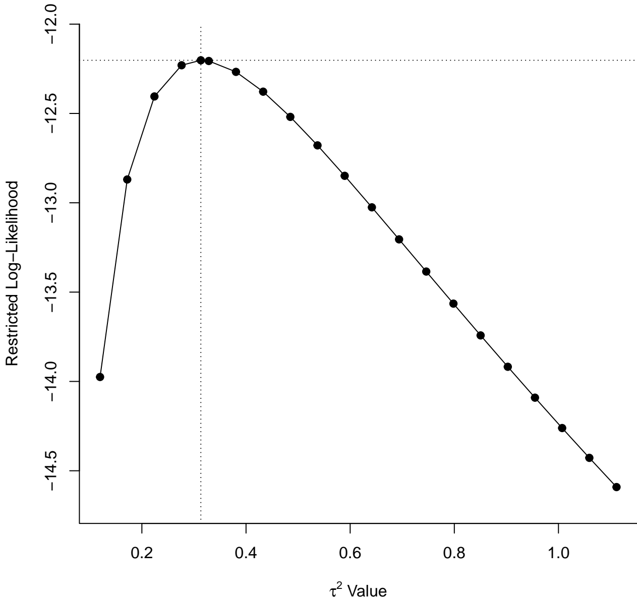
Profile Plot for \tau^2
