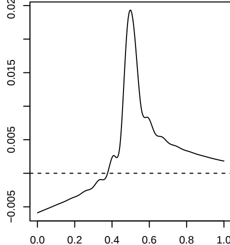
PC 2 Variability: 0 % of 30.63 %
