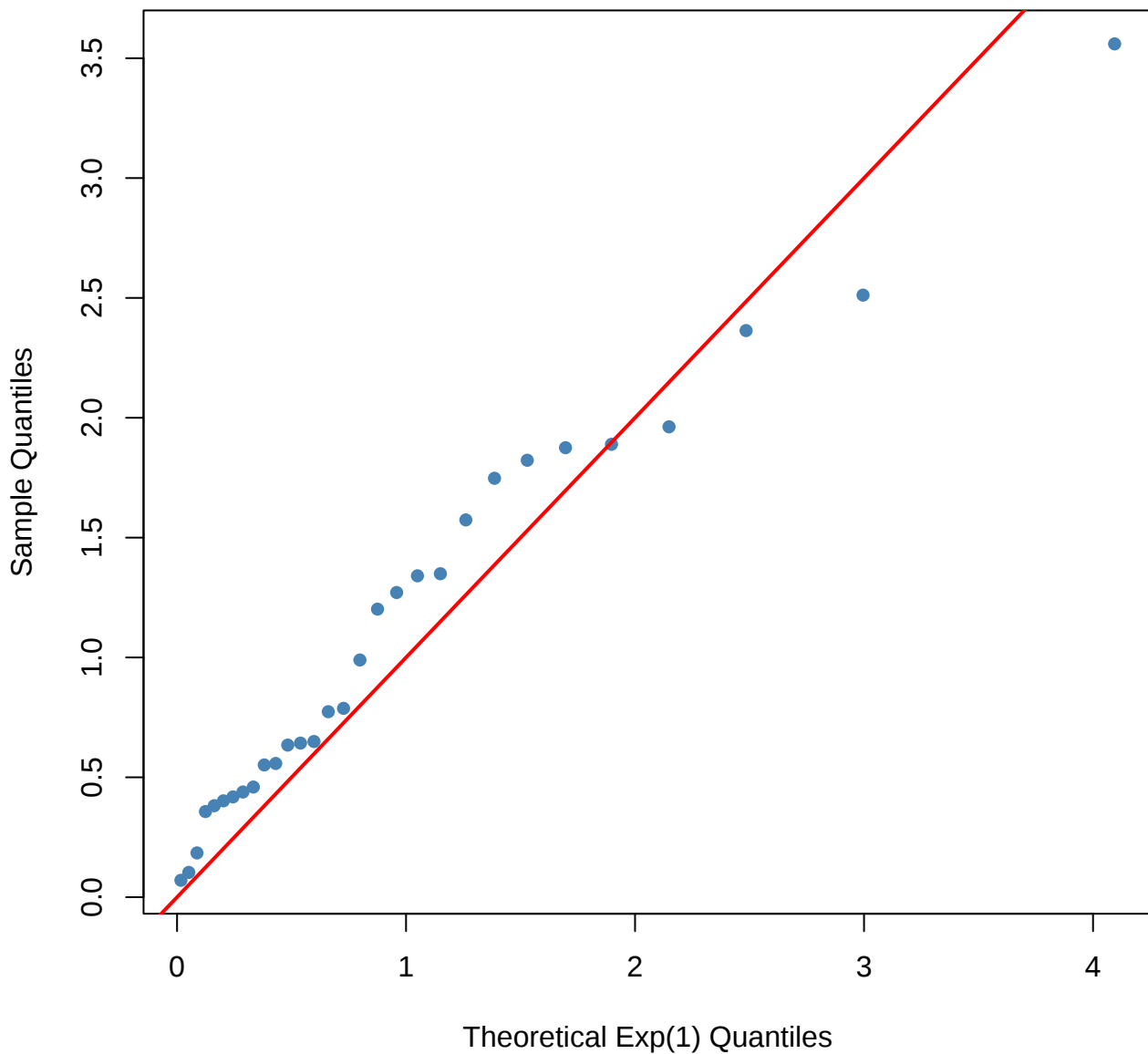
Cox-Snell Residuals Q-Q Plot
