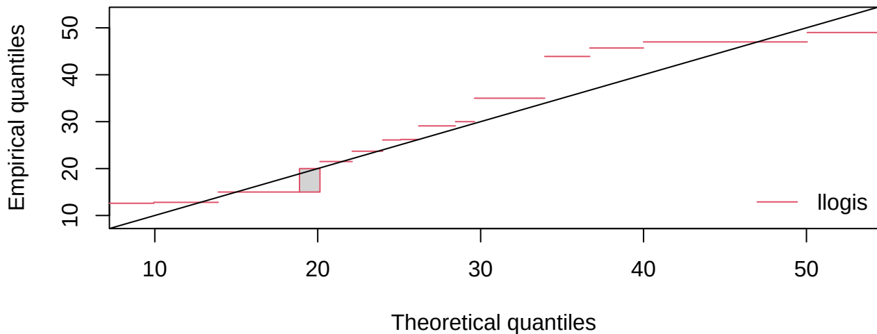
Q-Q plot
