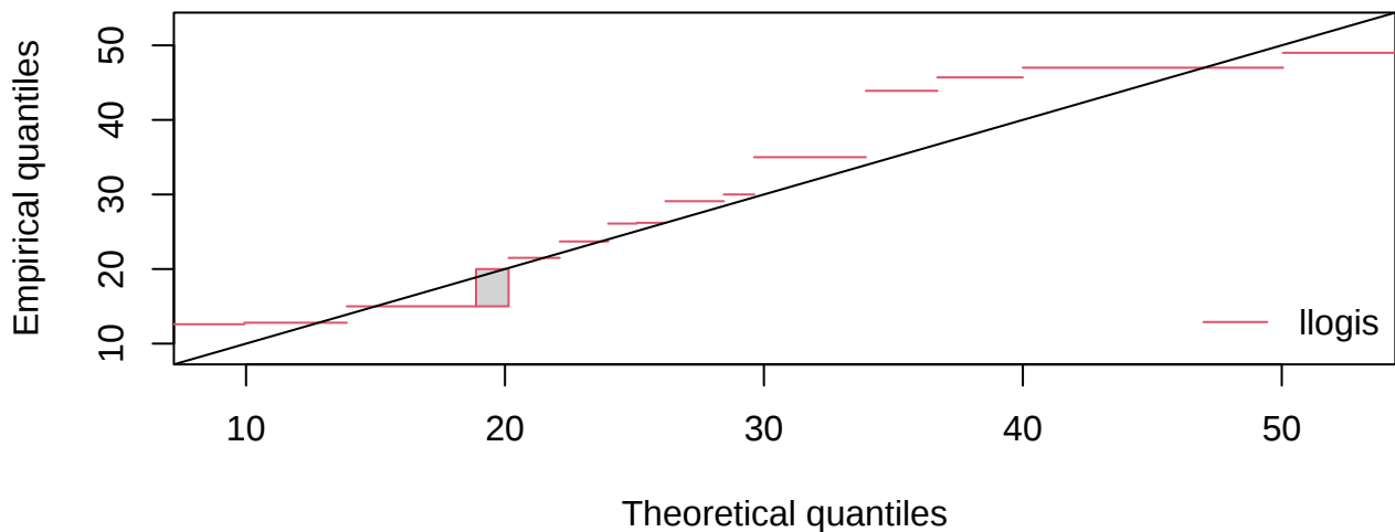
Q-Q plot
