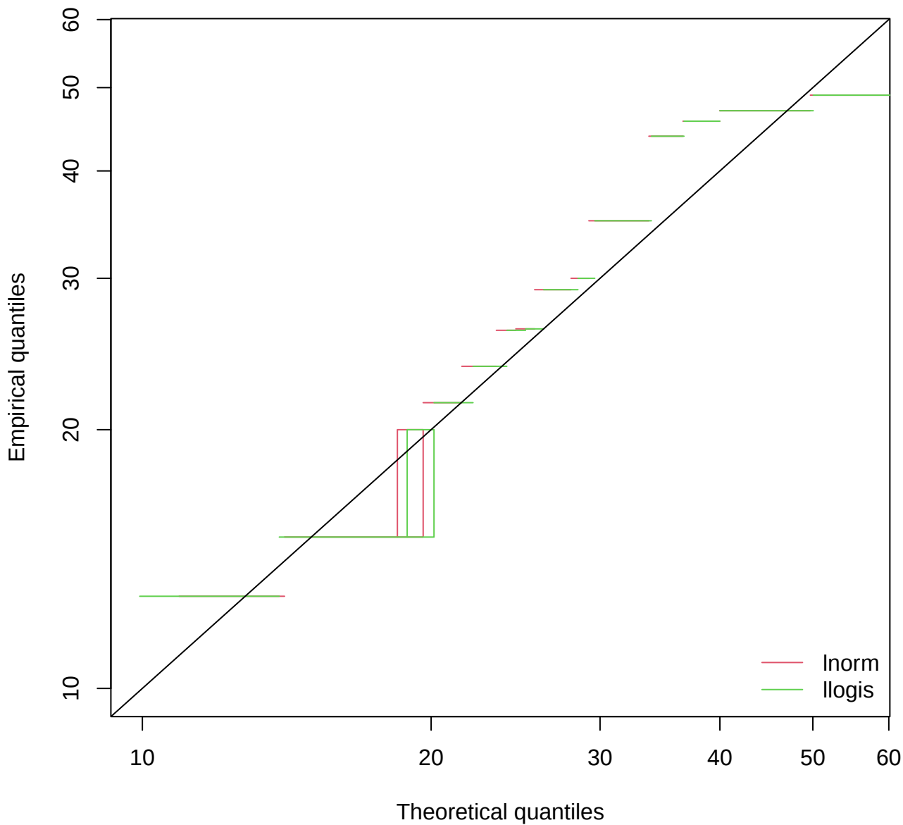
Q-Q plot
