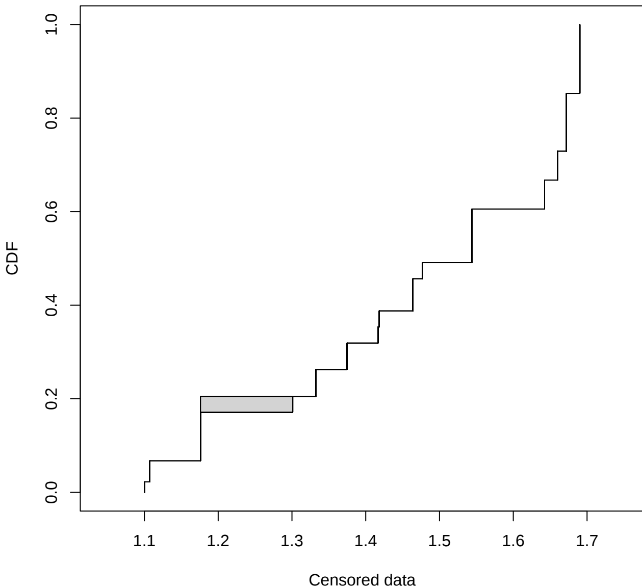
Cumulative distribution
