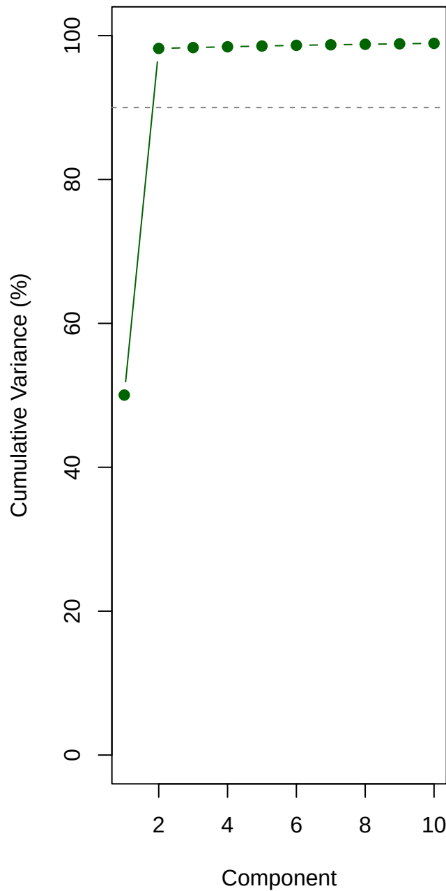
Explained Variance
