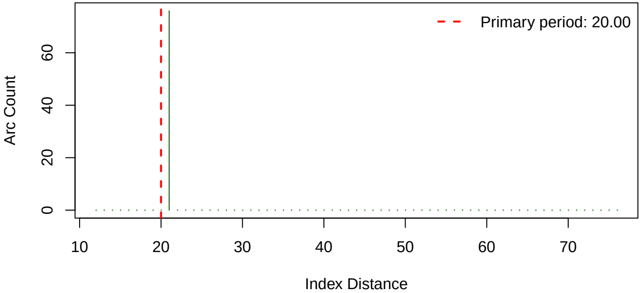
Arc Counts (for Period Detection)
