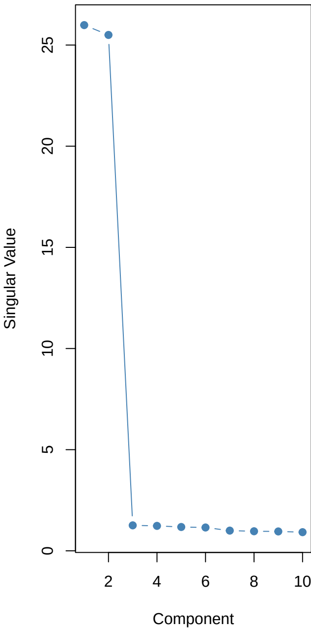
Singular Value Spectrum
