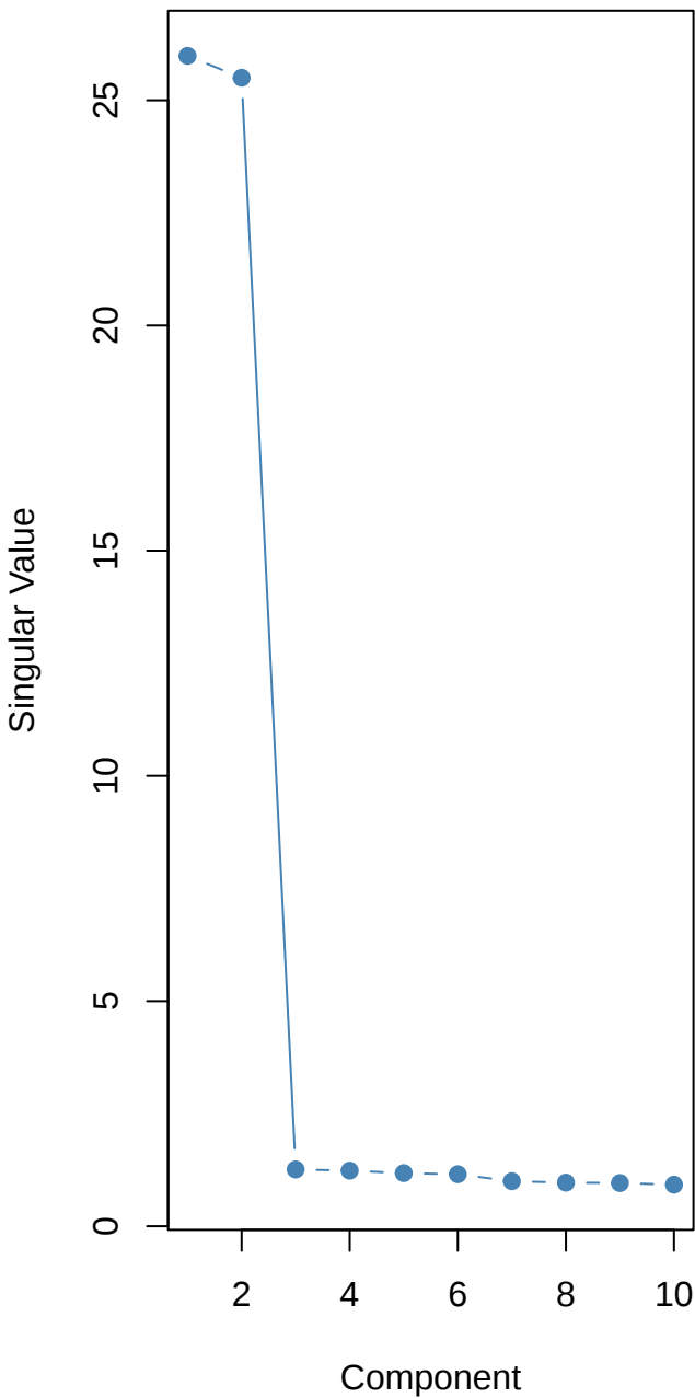
Singular Value Spectrum
