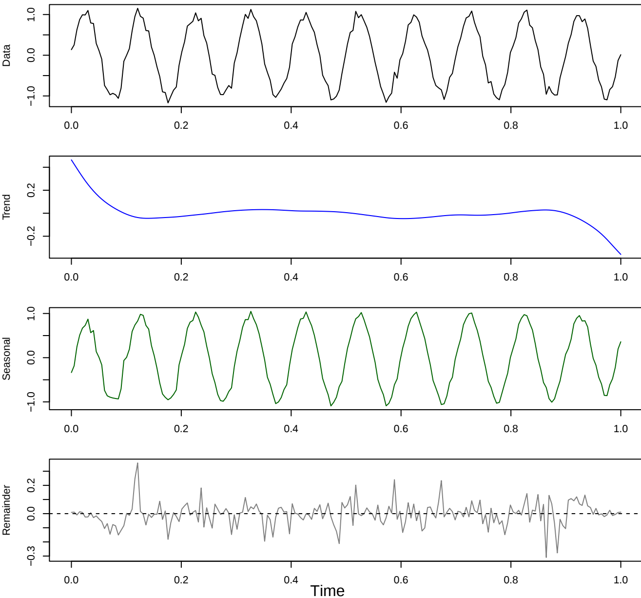
STL Decomposition – Curve 1
