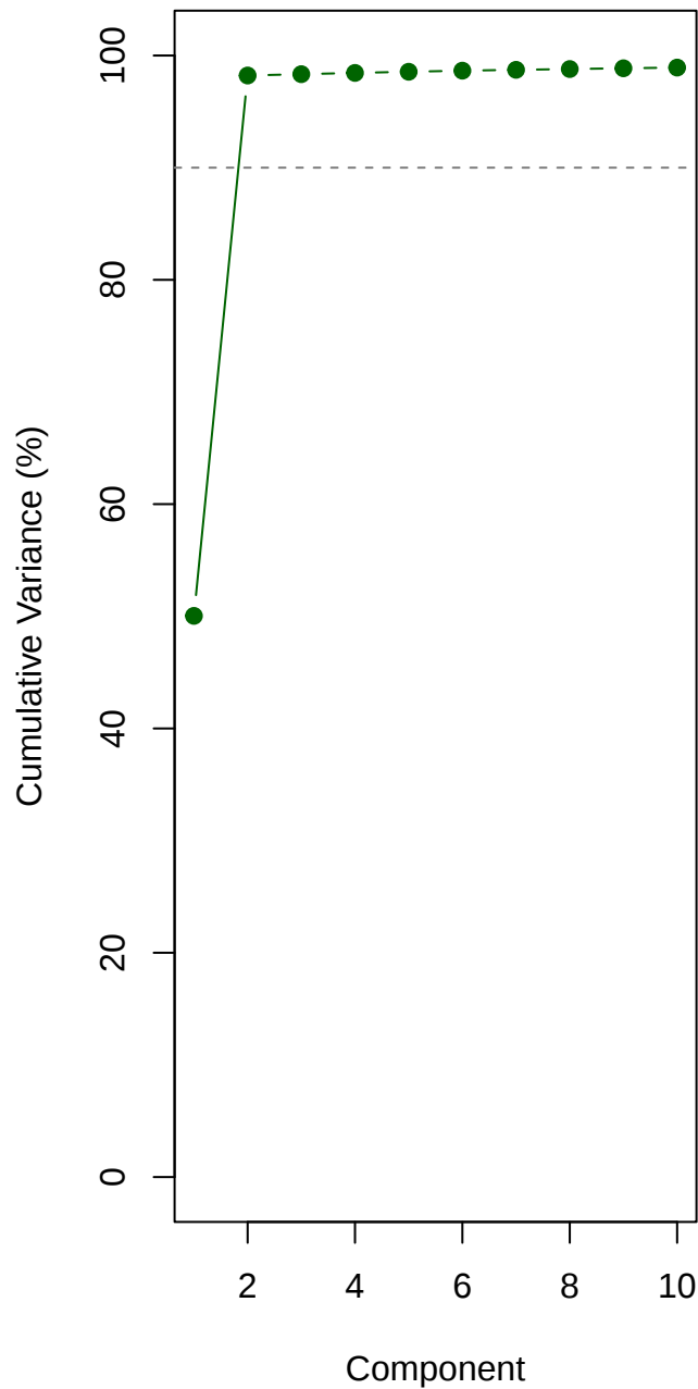
Explained Variance
