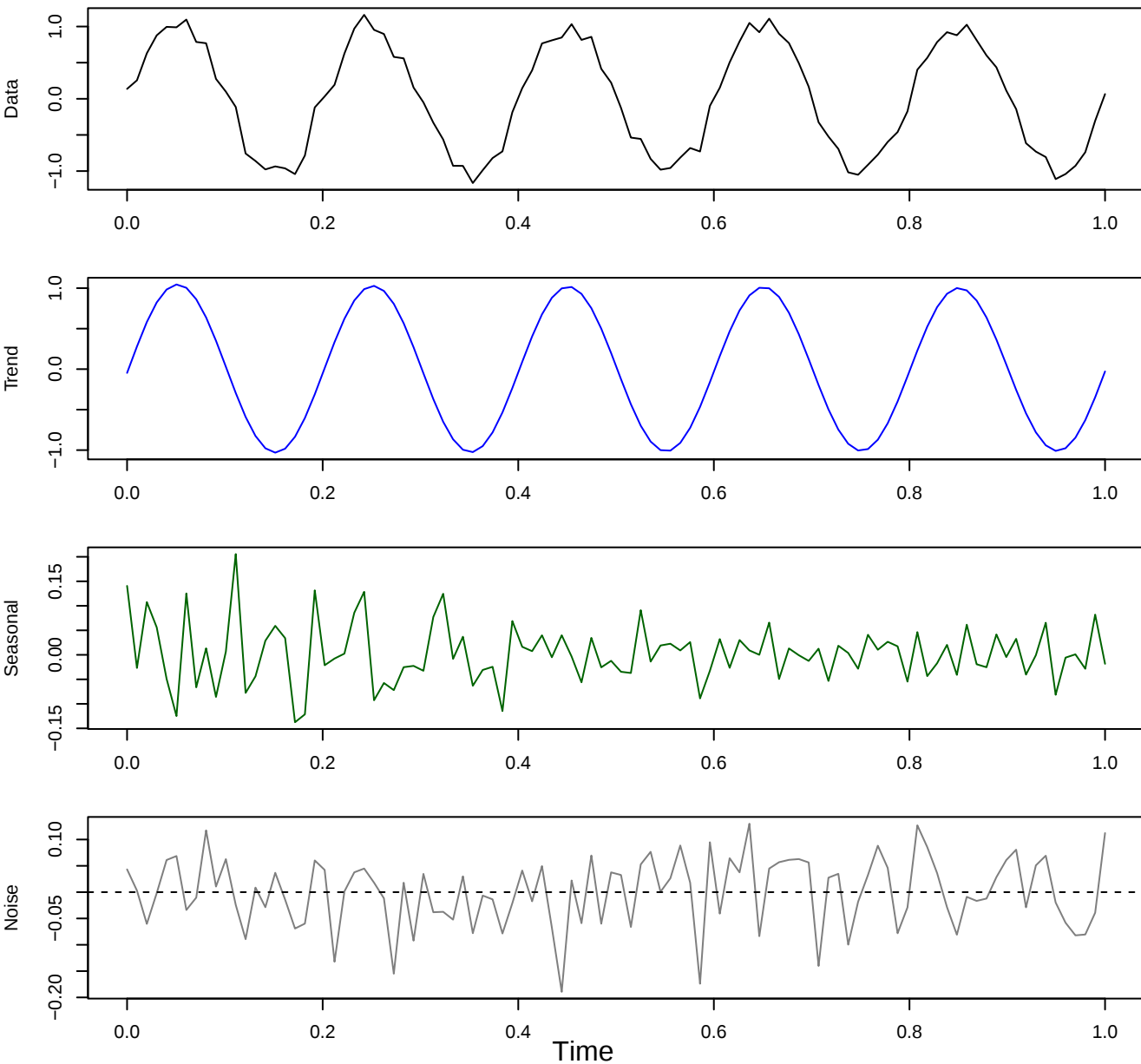
SSA Decomposition – Curve 1
