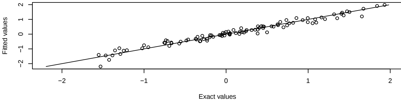
Leave-one-out
