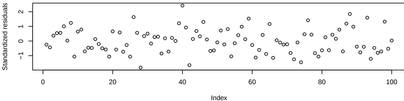
Standardized residuals
