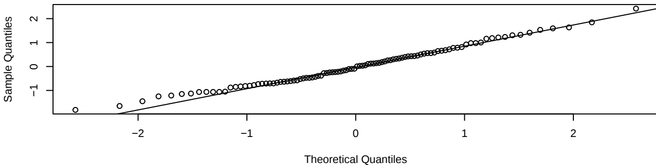
Normal QQ-plot of standardized residuals
