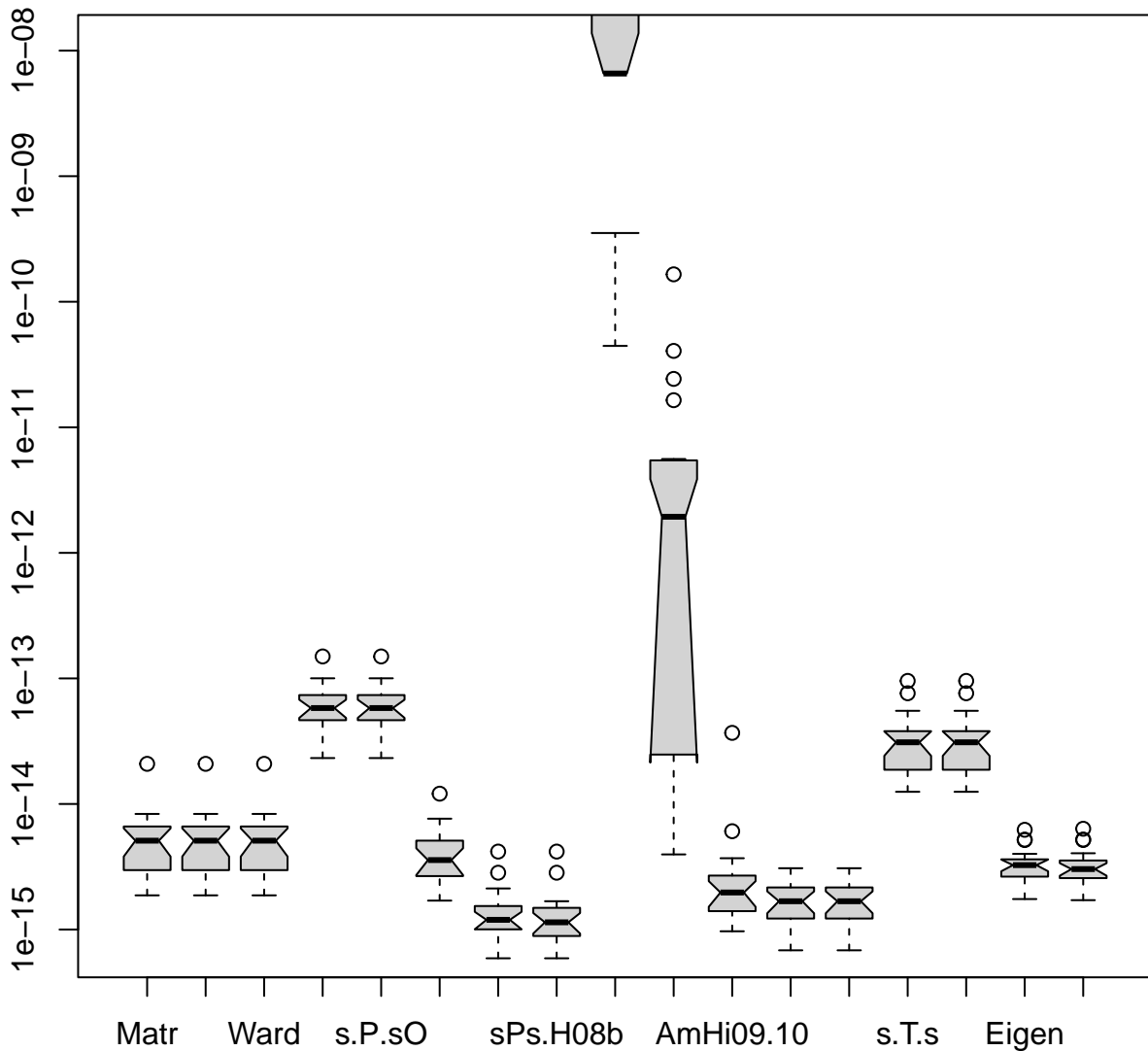
relative errors for 'random' eigen-ok 20 x 20 matrix
