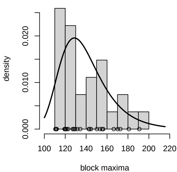
density plot
