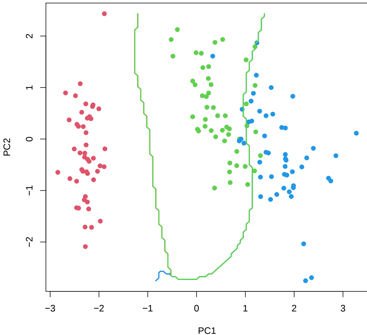
SVM Decision Boundary (PCA)
