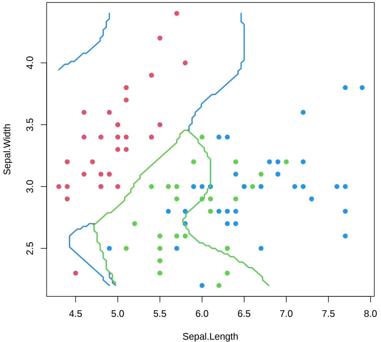
SVM Decision Boundary
