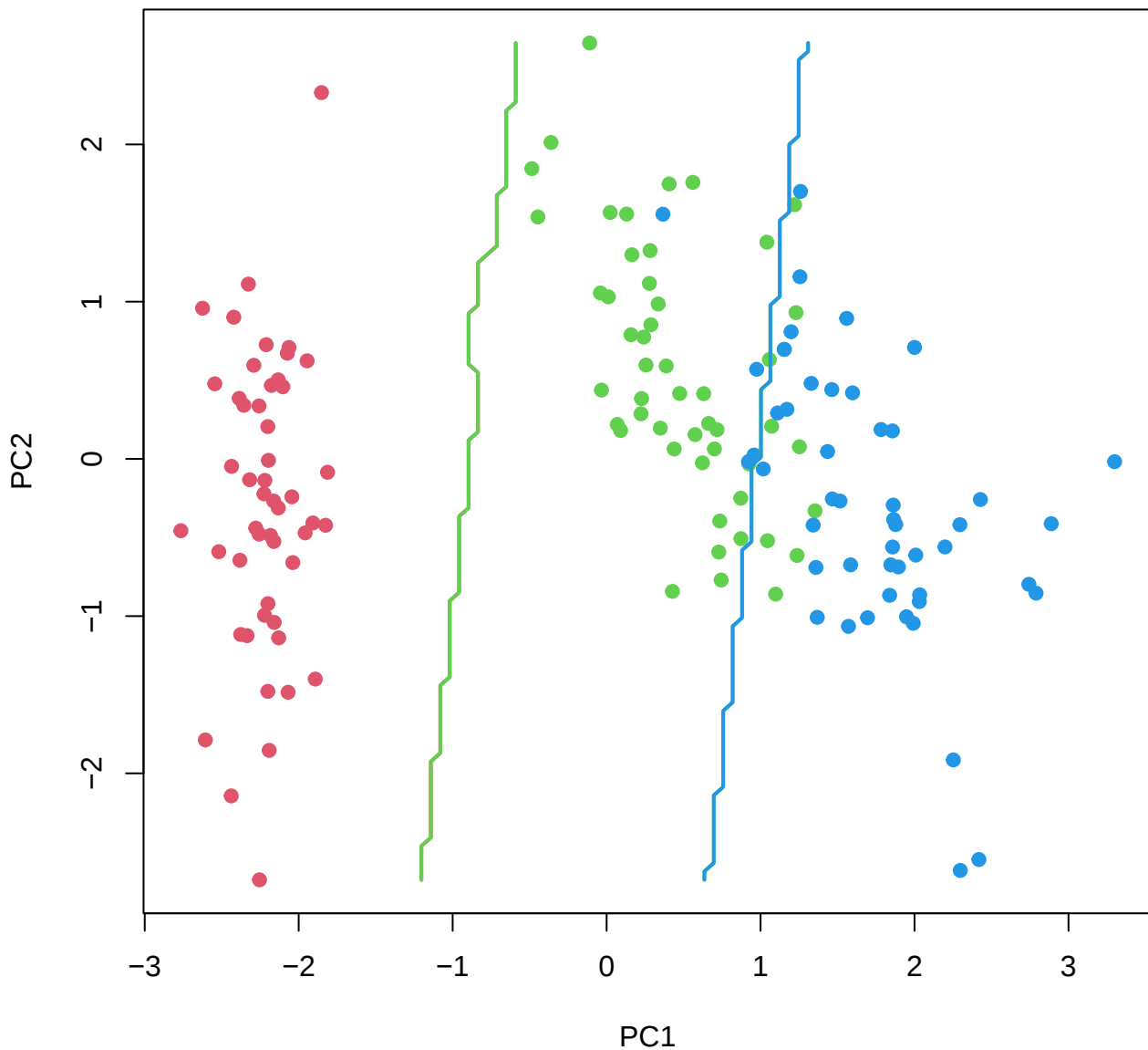
Random Forest Decision Boundary (PCA)
