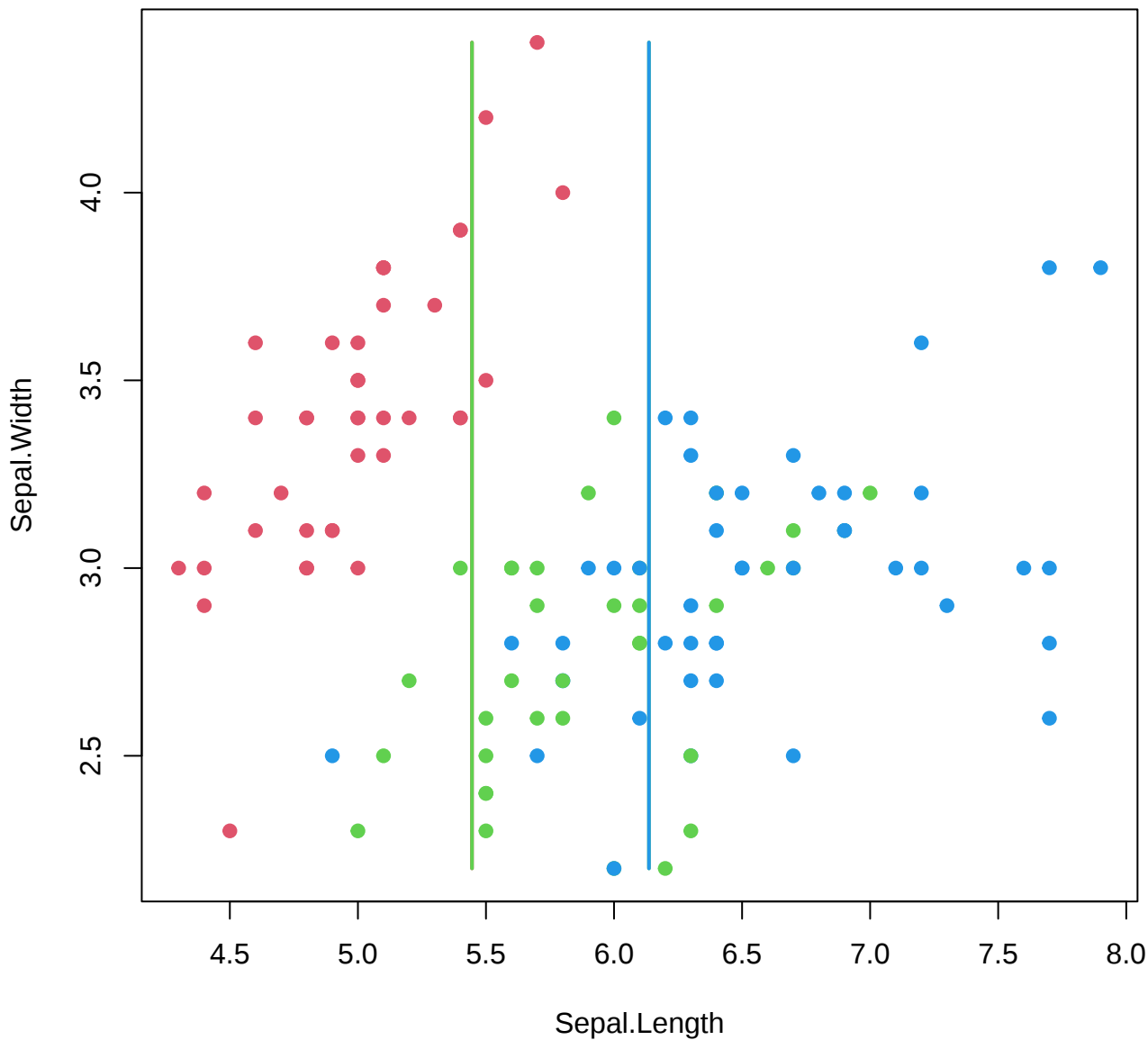
Decision Tree Decision Boundary
