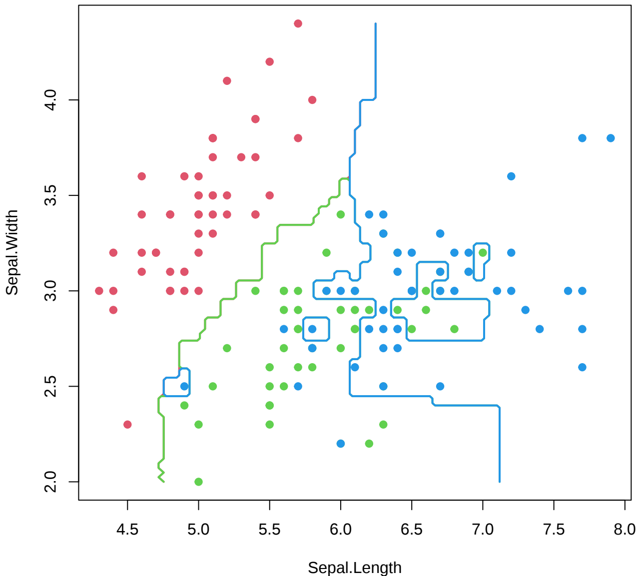
Random Forest Decision Boundary
