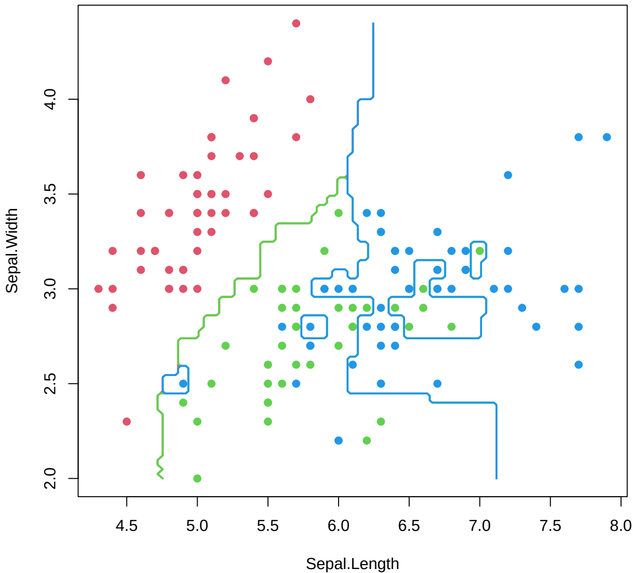
Random Forest Decision Boundary
