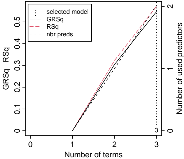
Model Selection (all responses)
