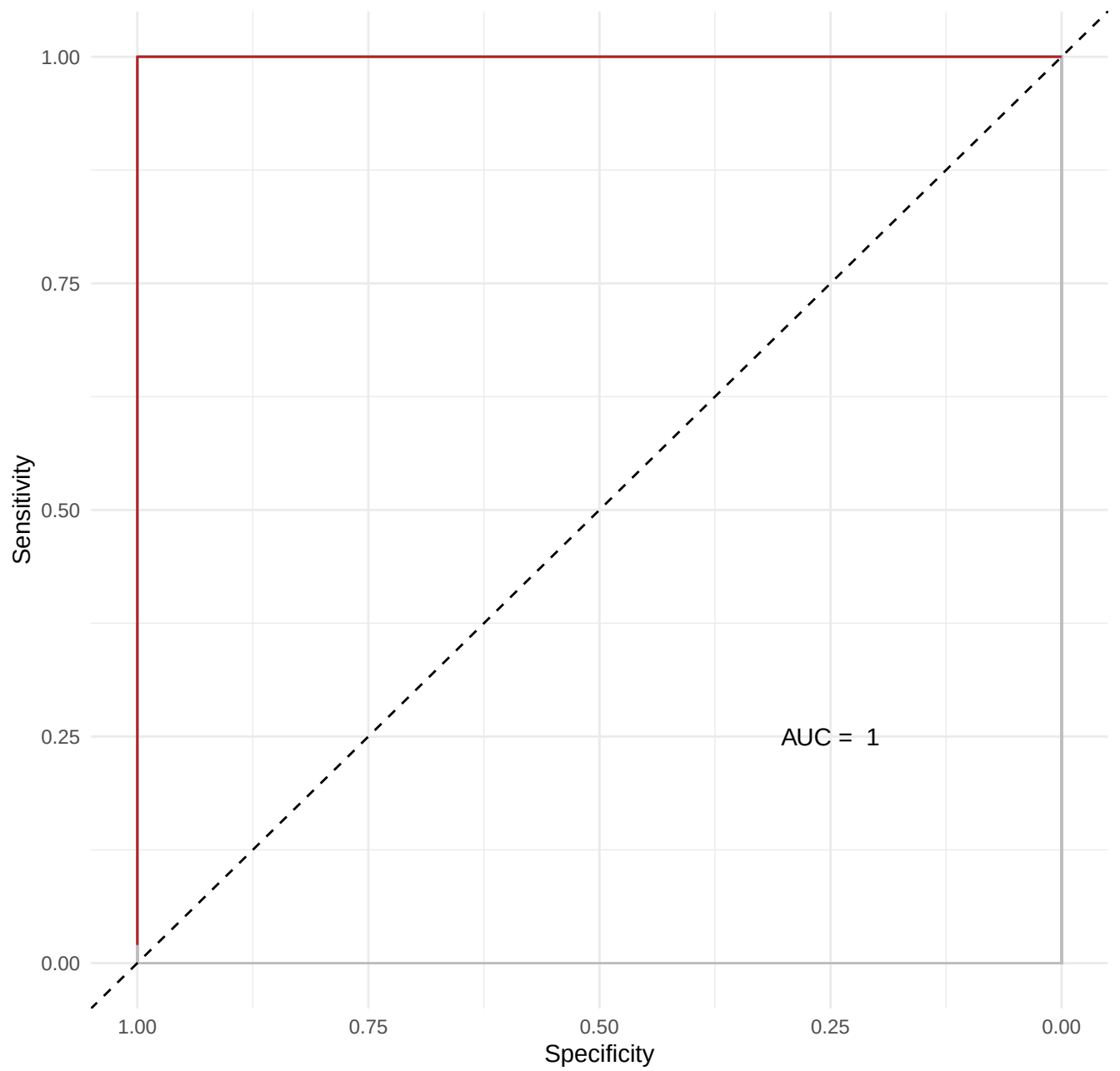
Roc Curve
