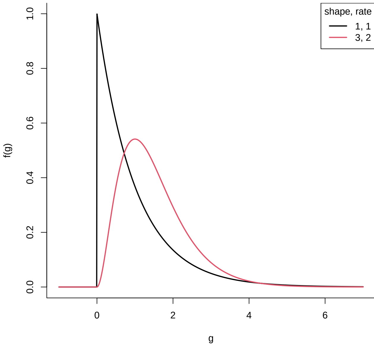
Gamma (shape, rate) p.d.f.
