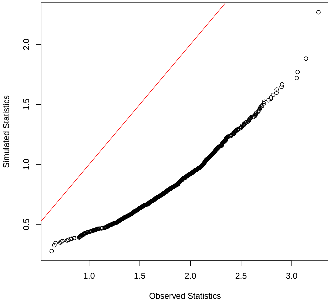
Q-Q Plot for KS (n=100, reps=1000)
