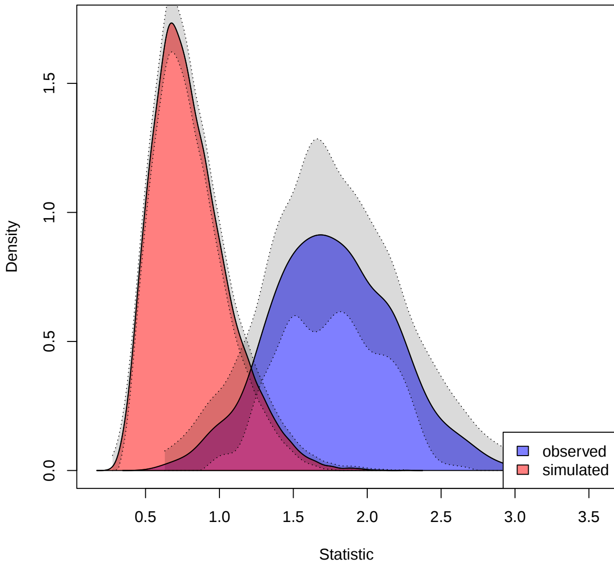
Observed and simulated KS Densities (n=100, reps=1000)
