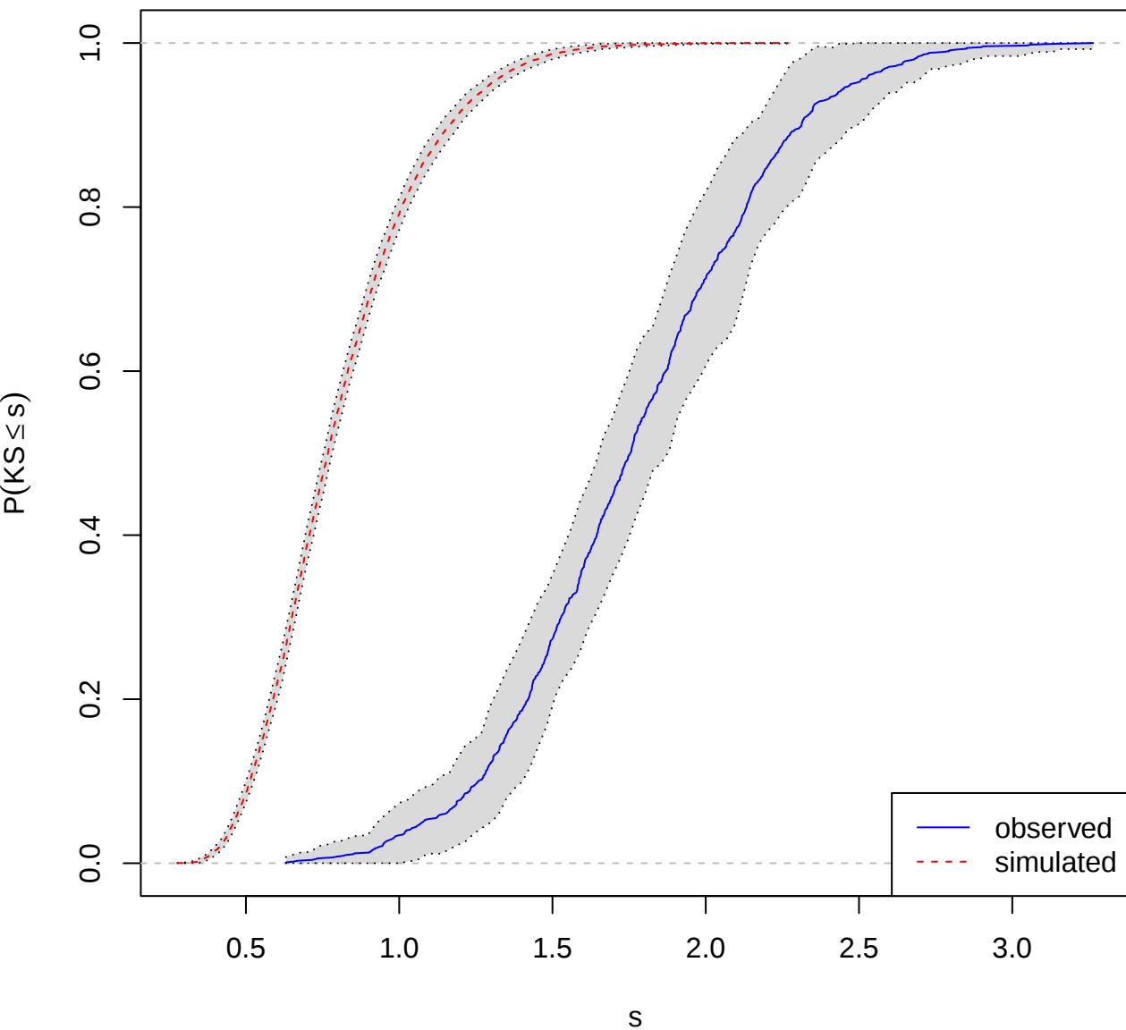
Observed and simulated KS CDFs (n=100, reps=1000)
