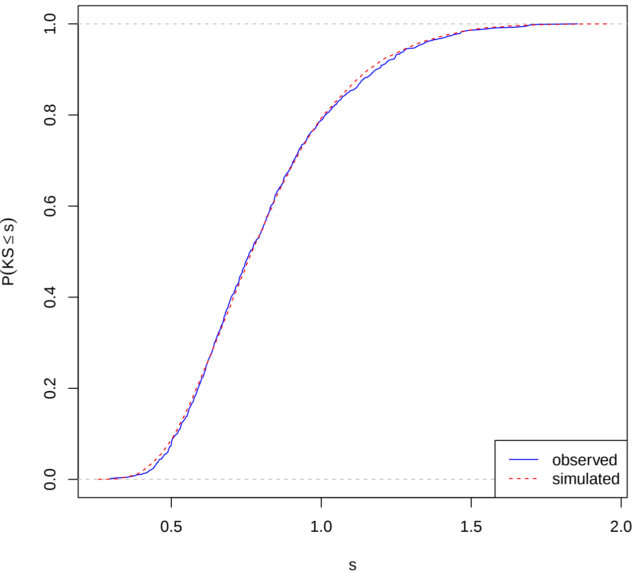
Observed and simulated KS CDFs (n=100, reps=1000)
