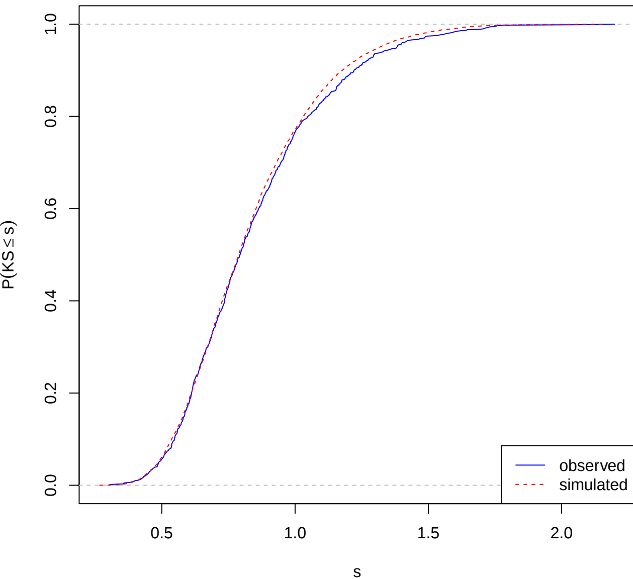
Observed and simulated KS CDFs (n=300, reps=1000)
