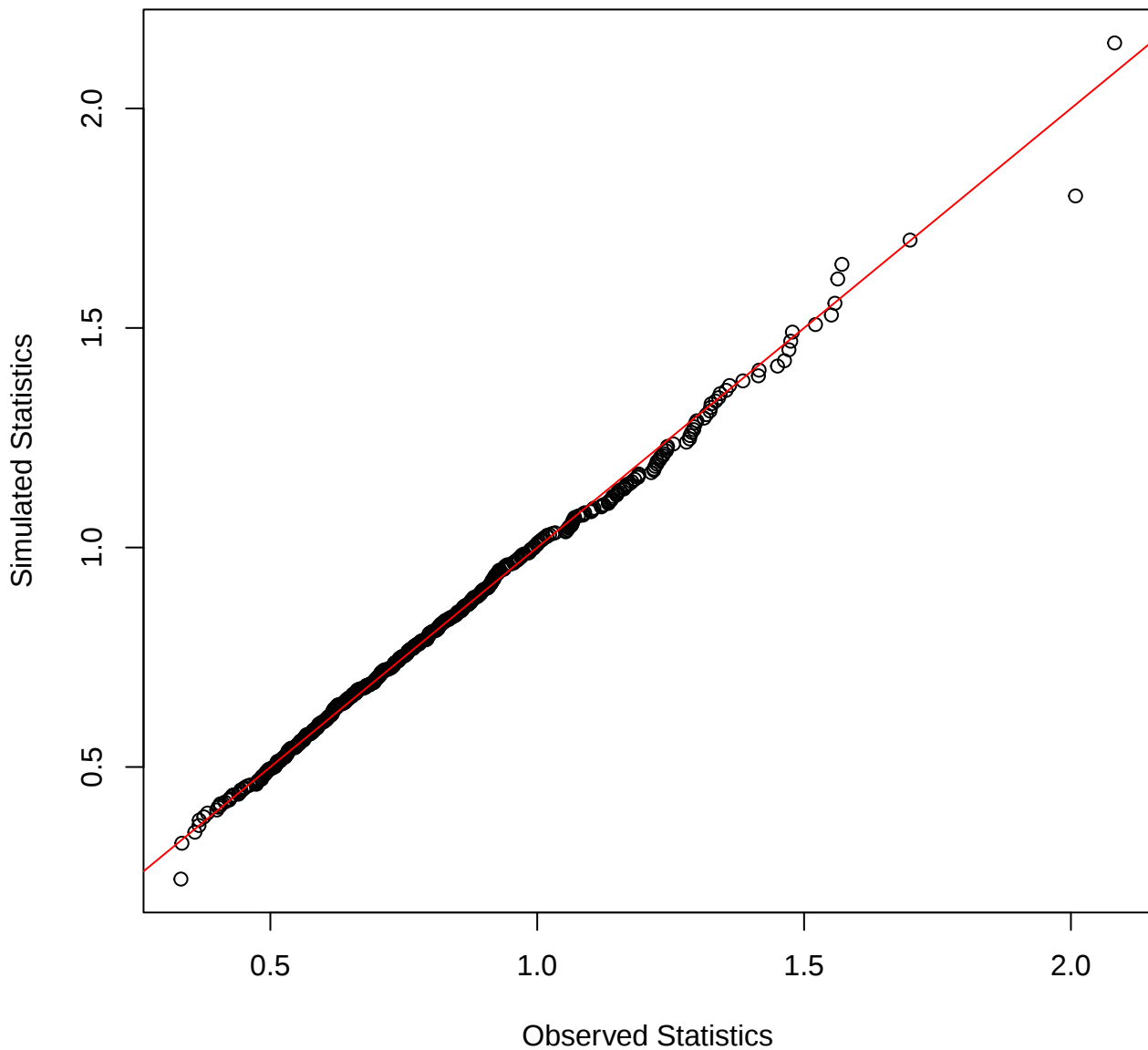
Q-Q Plot for KS (n=100, reps=500)
