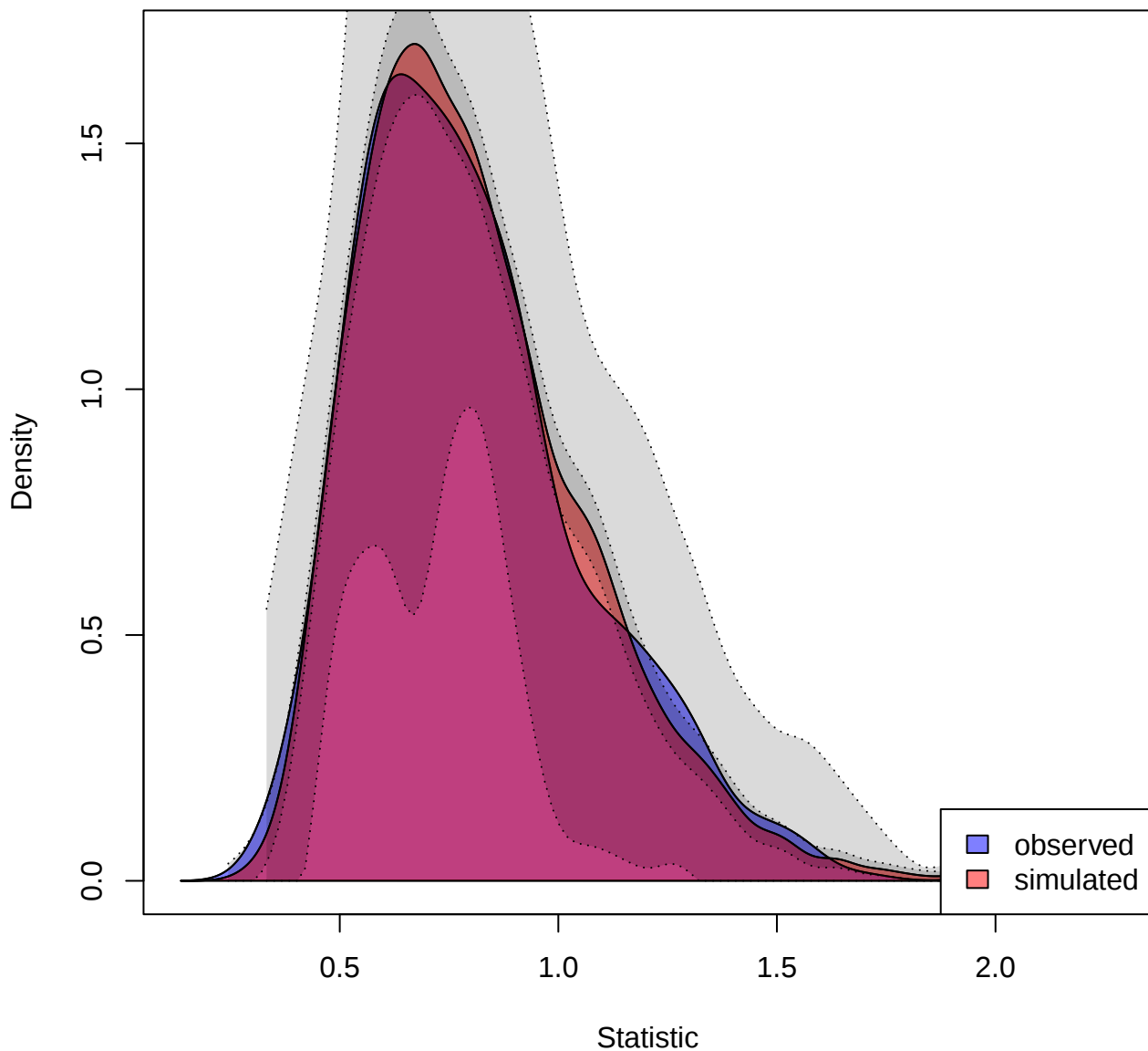
Observed and simulated KS Densities (n=100, reps=500)
