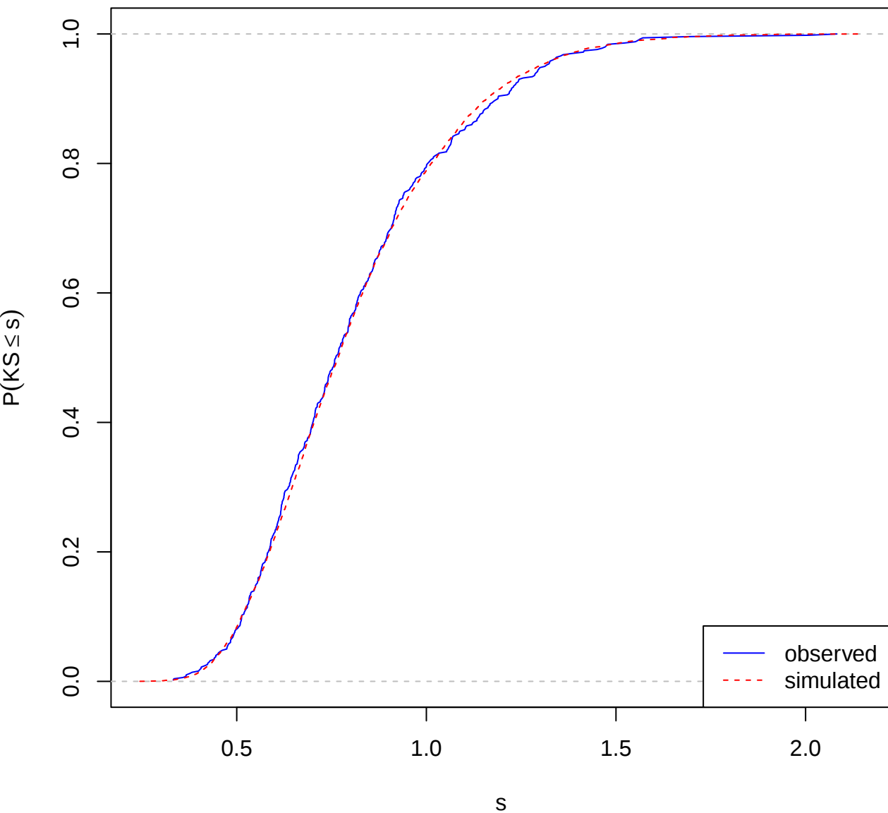
Observed and simulated KS CDFs (n=100, reps=500)
