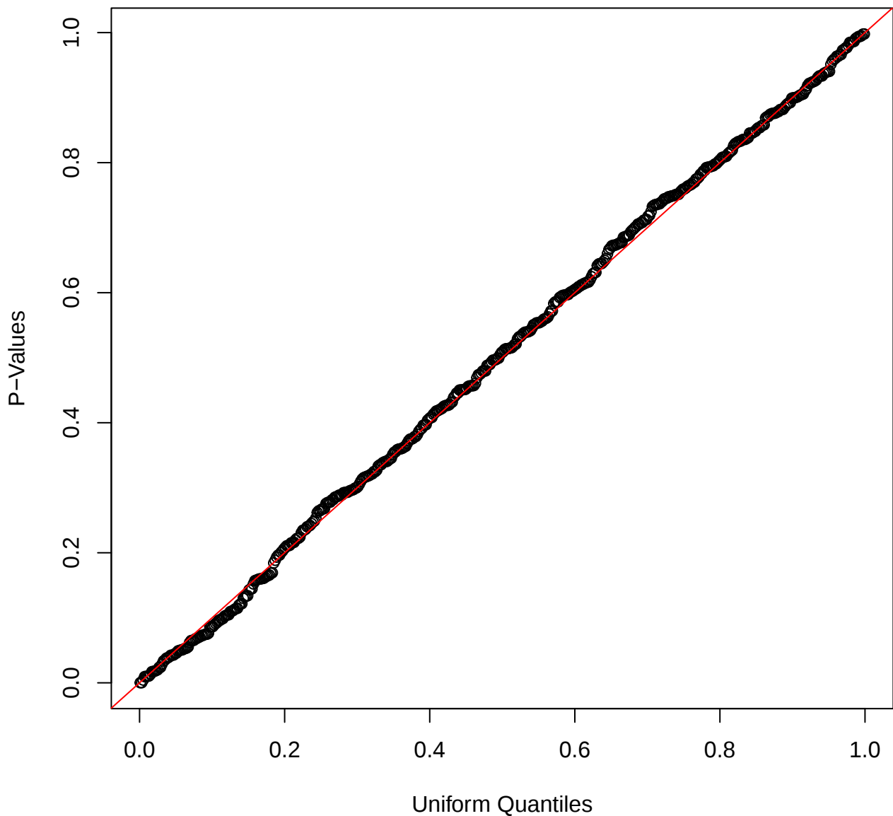
P-Values and Uniform Quantiles for KS (n=100, reps=500)
