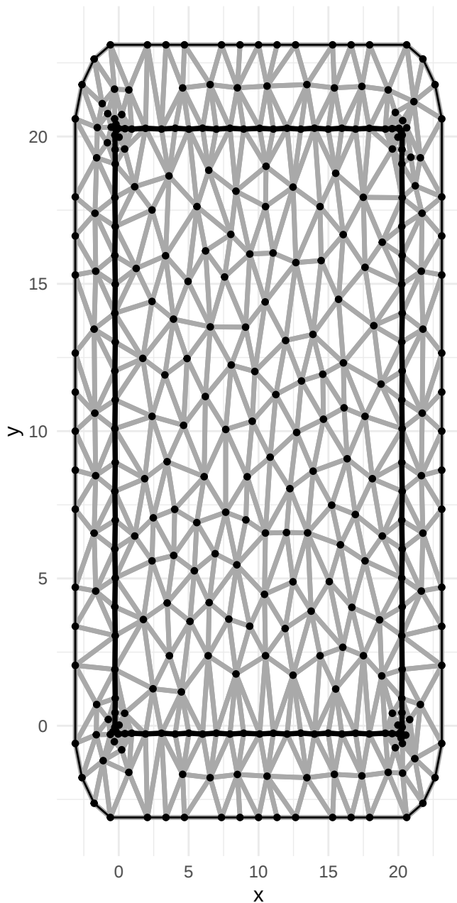
INLA mesh for spatial field
