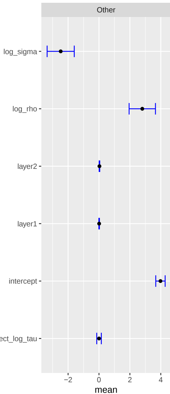
Parameters (excluding random)
