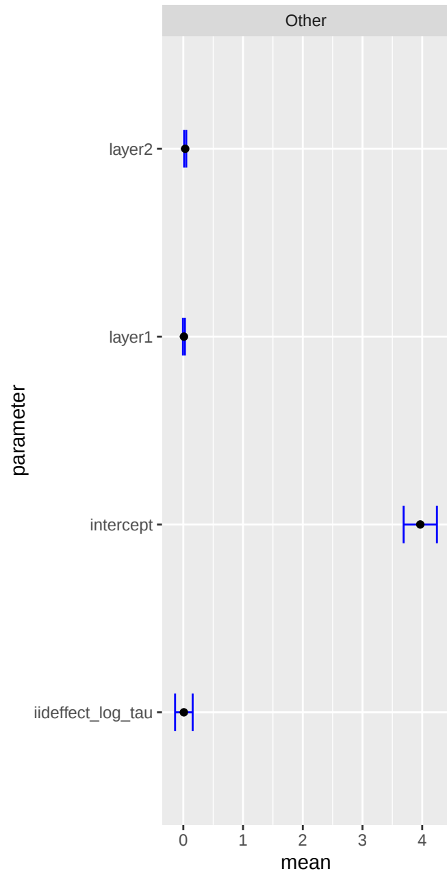
Parameters (excluding random)
