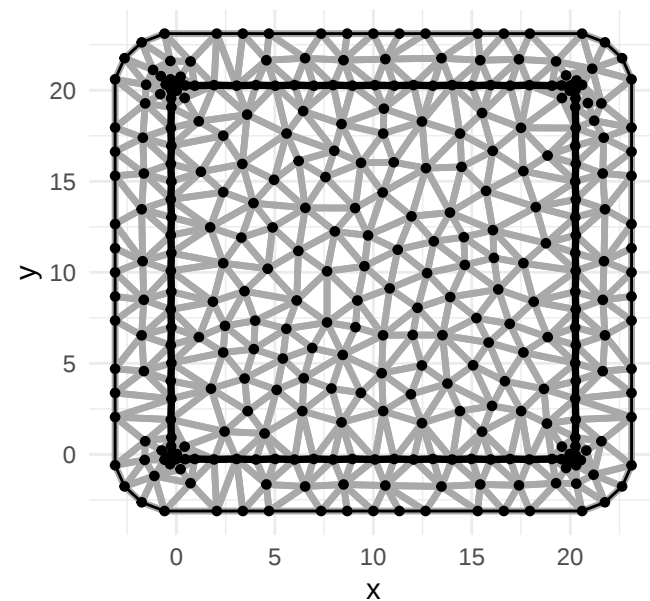
INLA mesh for spatial field
