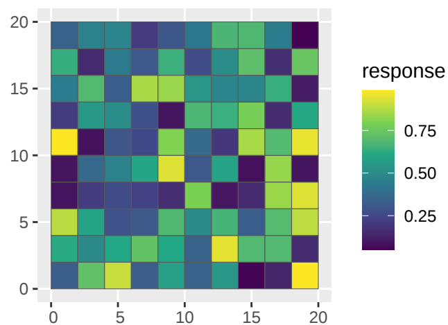
Polygon response data
