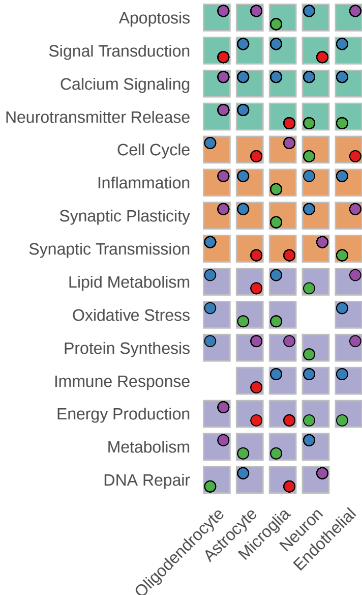
Dice Plot with Varying Counts
