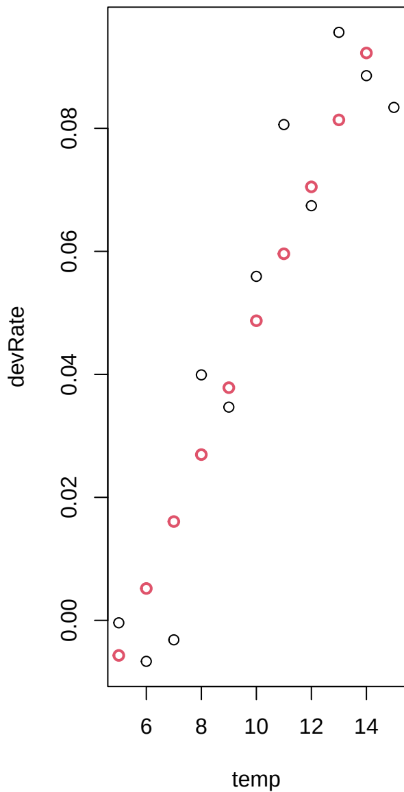
Obs. versus fitted (cor: 0.9366)
