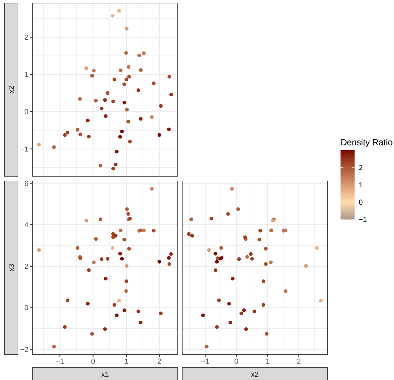
Scatter plots, with density ratio mapped to colour
