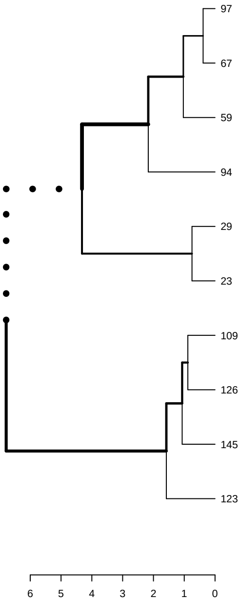
dendrogram1
