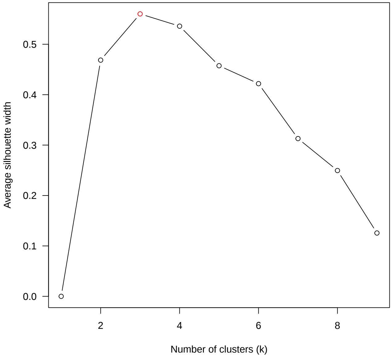
Estimating the number of clusters using average silhouette width
