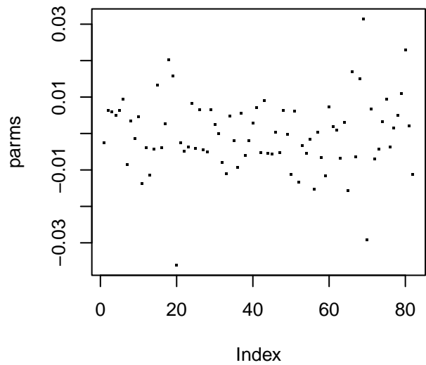
Network Weights
