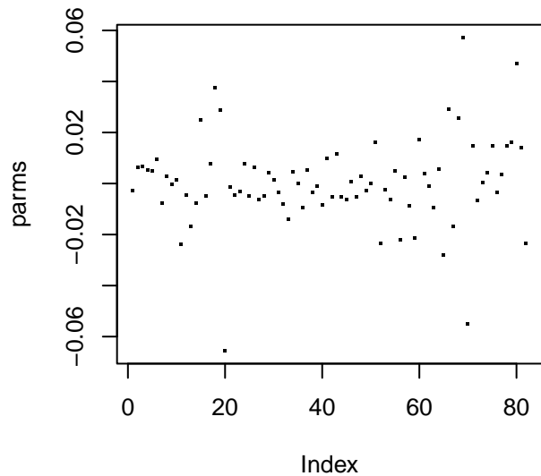
Network Weights
