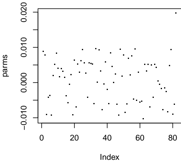
Network Weights
