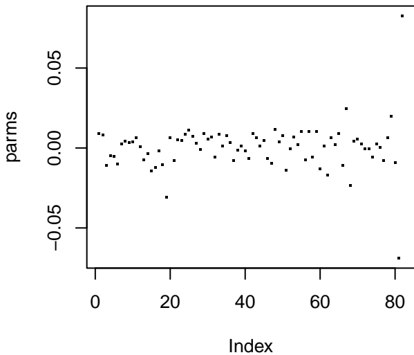
Network Weights
