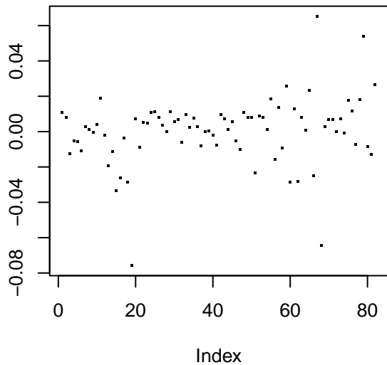
Network Weights
