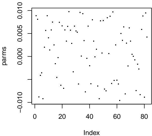
Network Weights
