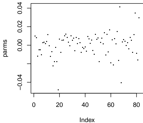
Network Weights
