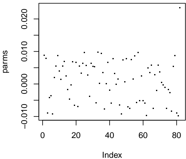
Network Weights
