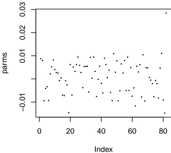
Network Weights
