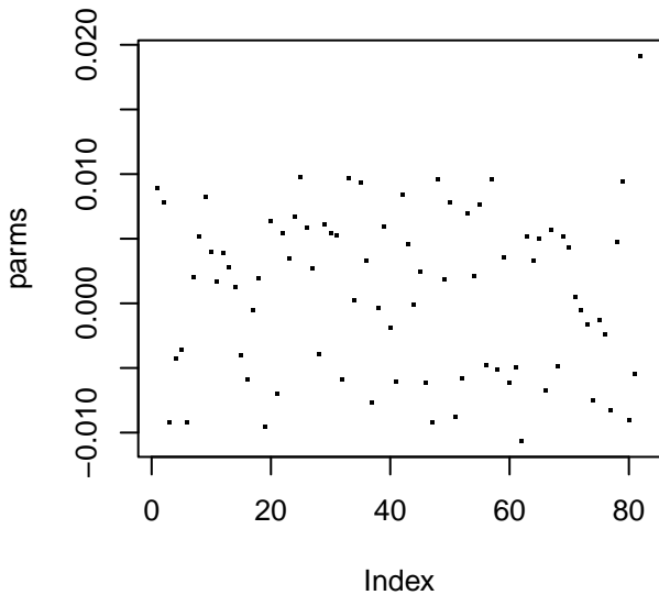
Network Weights
