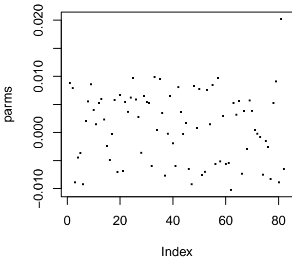
Network Weights
