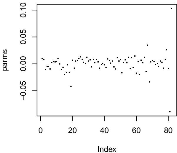
Network Weights
