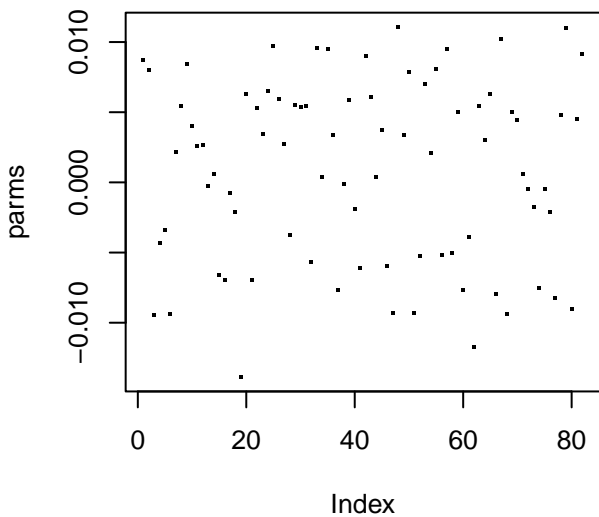
Network Weights
