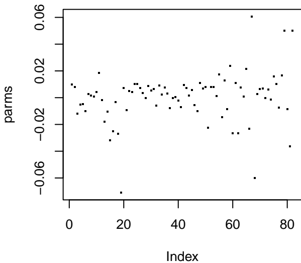
Network Weights
