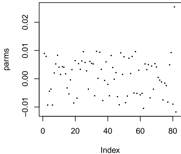
Network Weights
