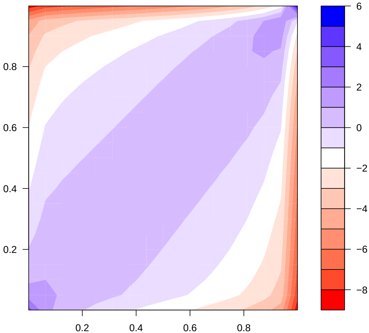
log Density( gumbelCopula(2) )
