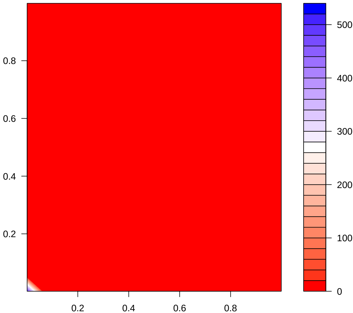
Density( claytonCopula(2) )
