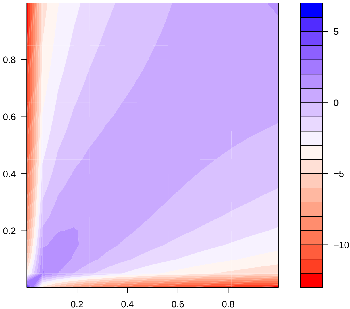
log Density( claytonCopula(2) )
