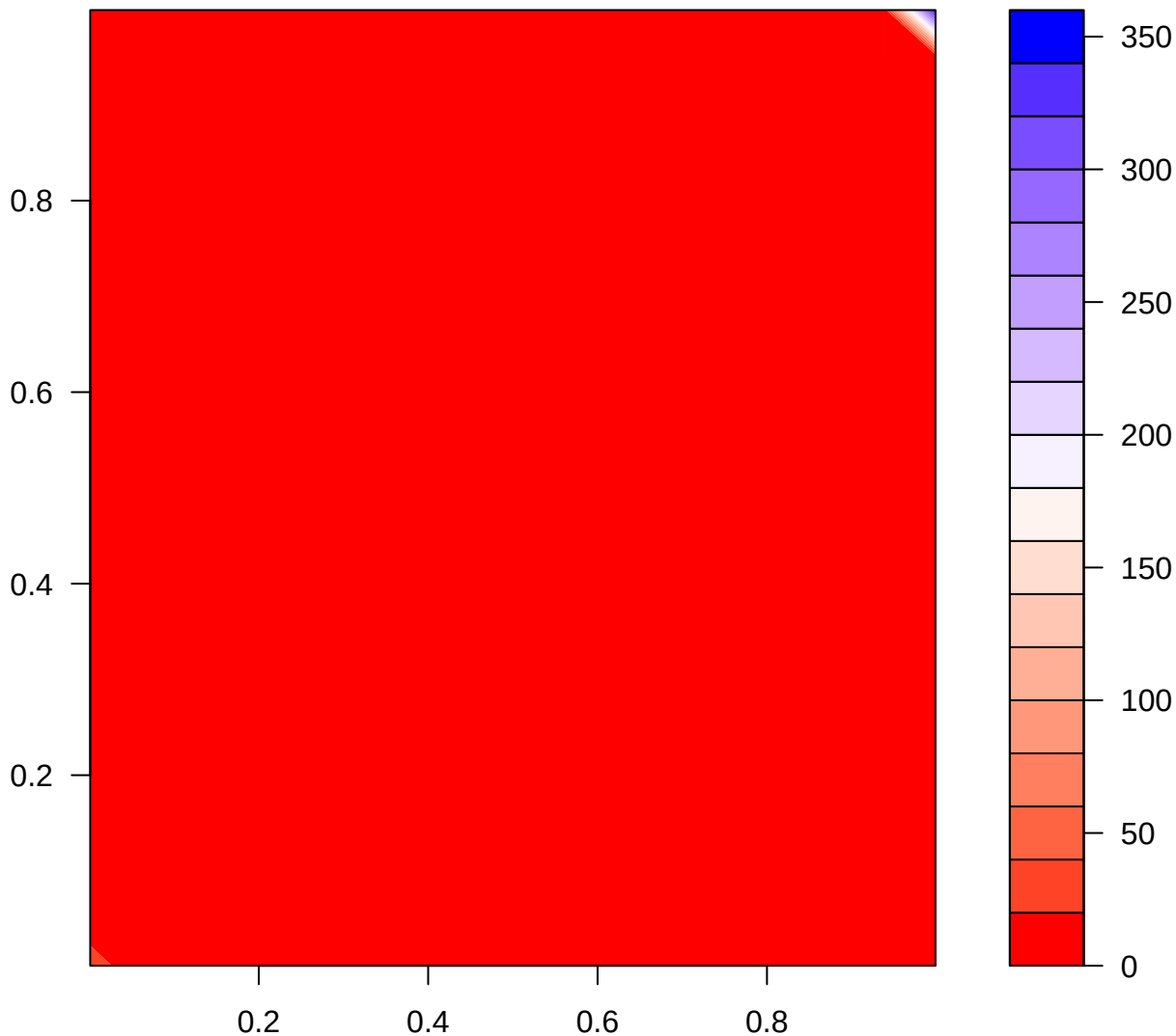
Density( gumbelCopula(2) )
