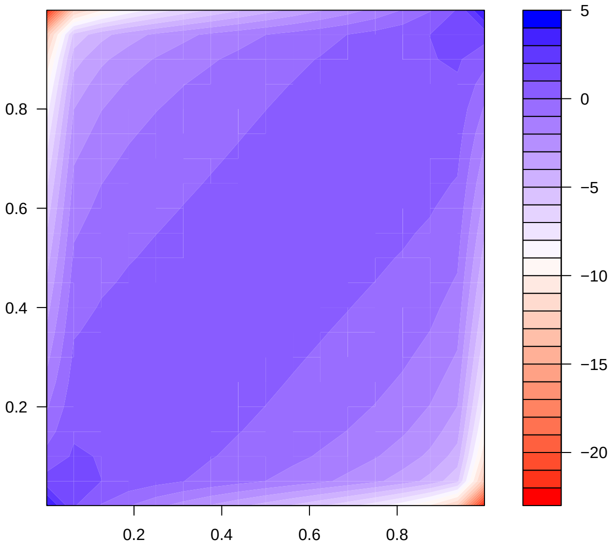
log Density( normalCopula(0.7071) )
