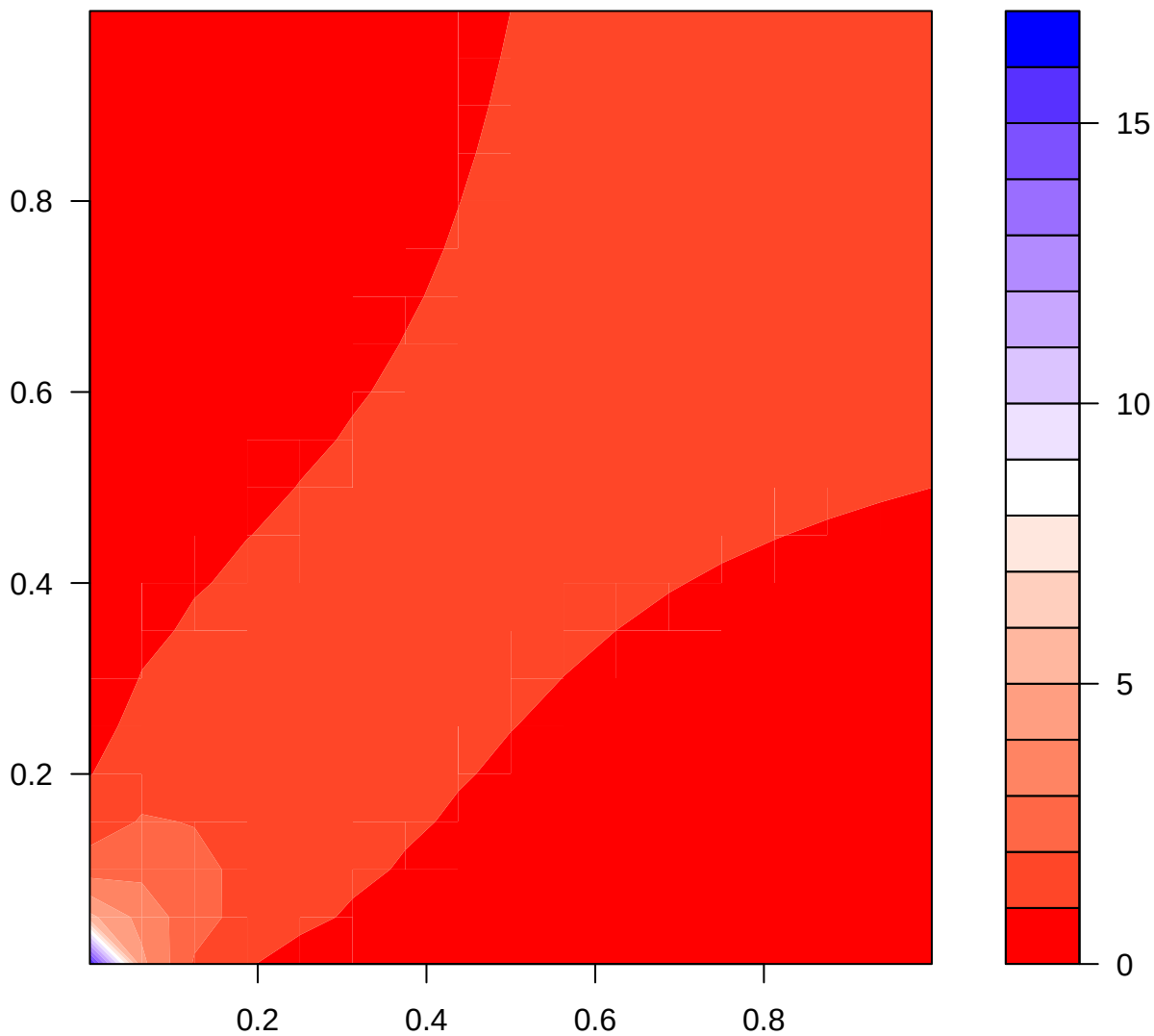
Density( amhCopula(0.943) )
