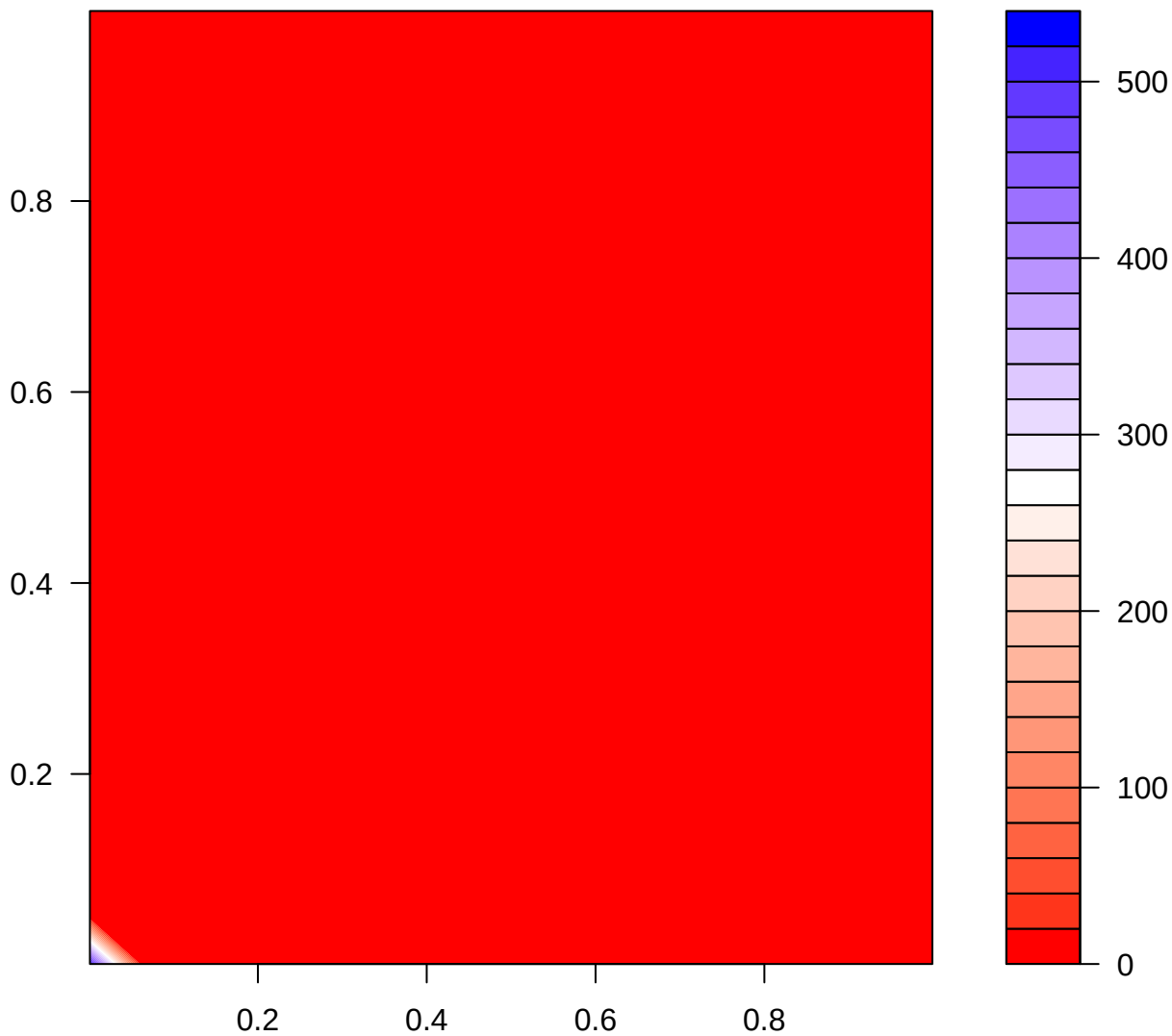
Density( claytonCopula(2) )
