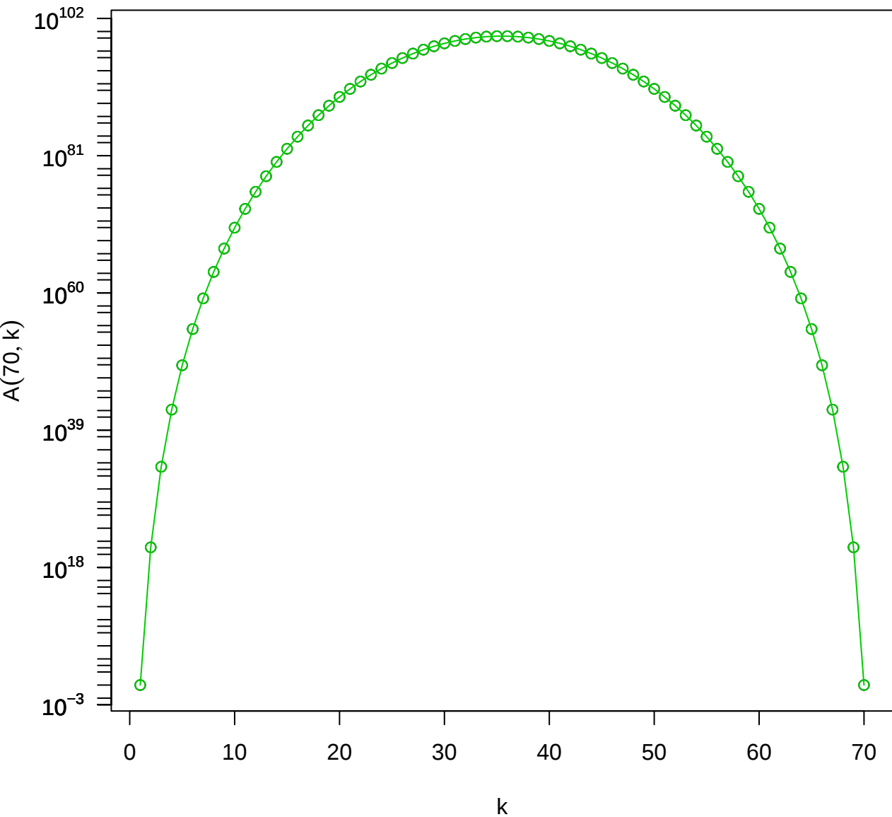
Eulerian numbers A(70, k)
