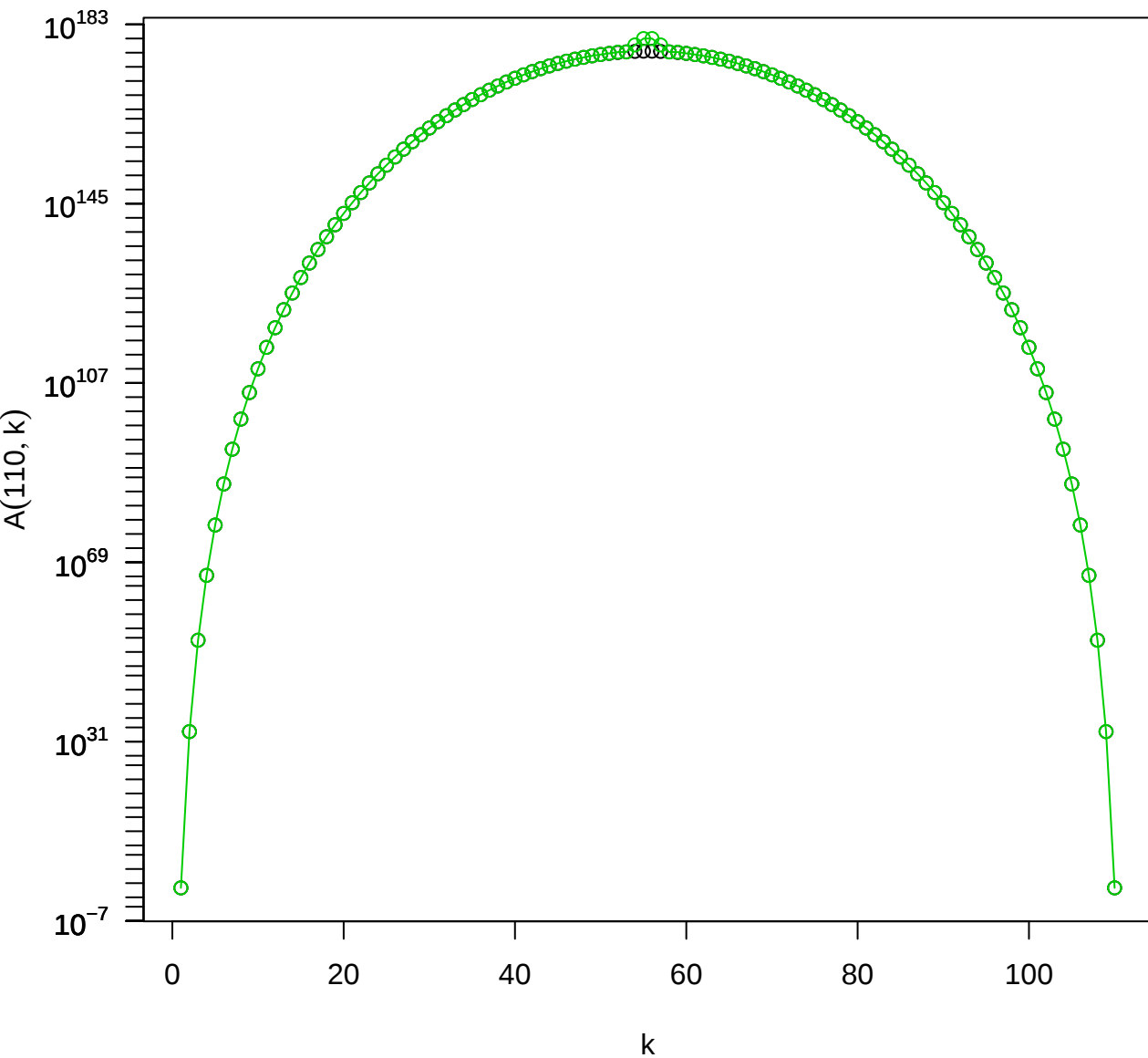
Eulerian numbers A(110, k)
