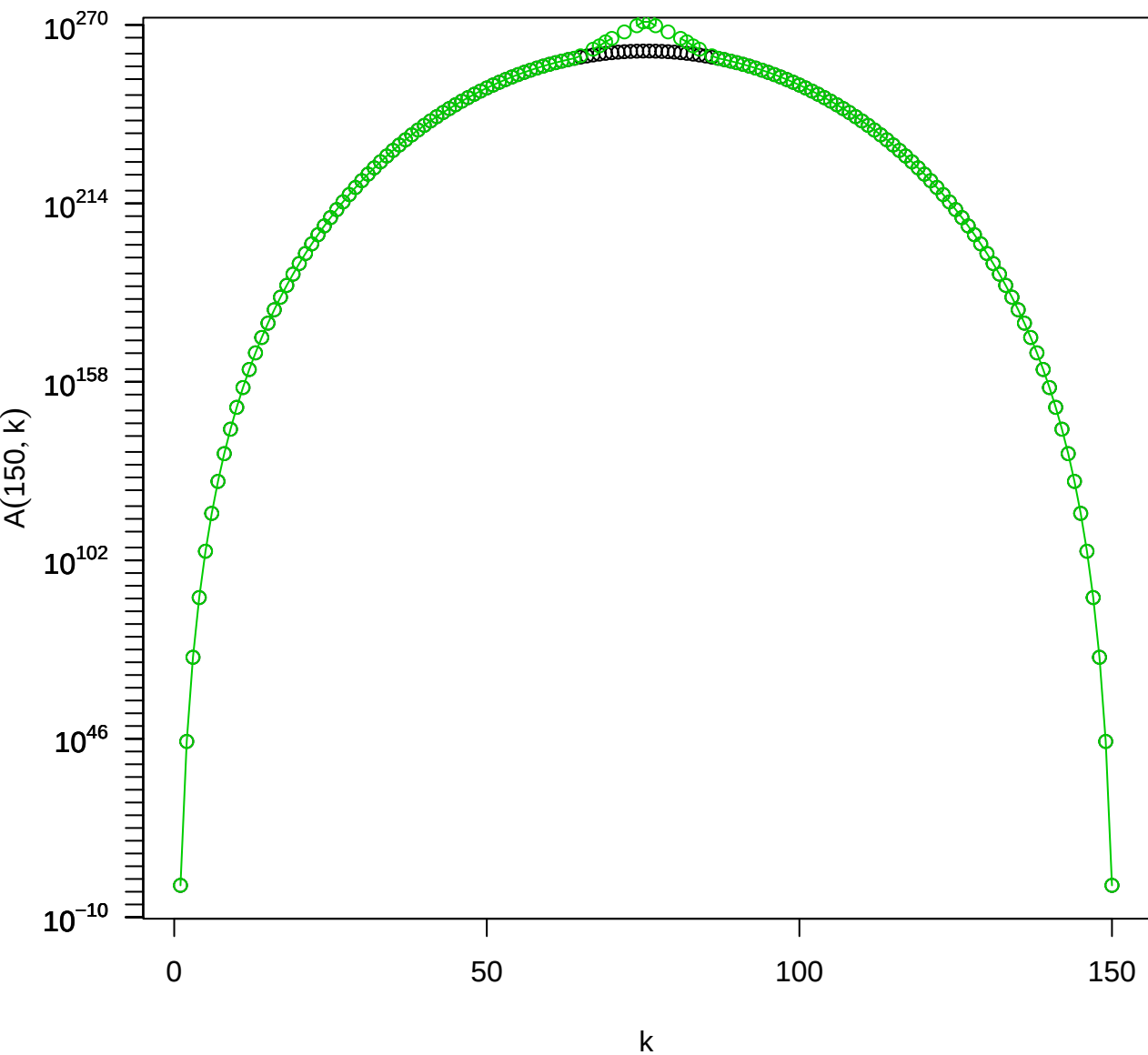
Eulerian numbers A(150, k)
