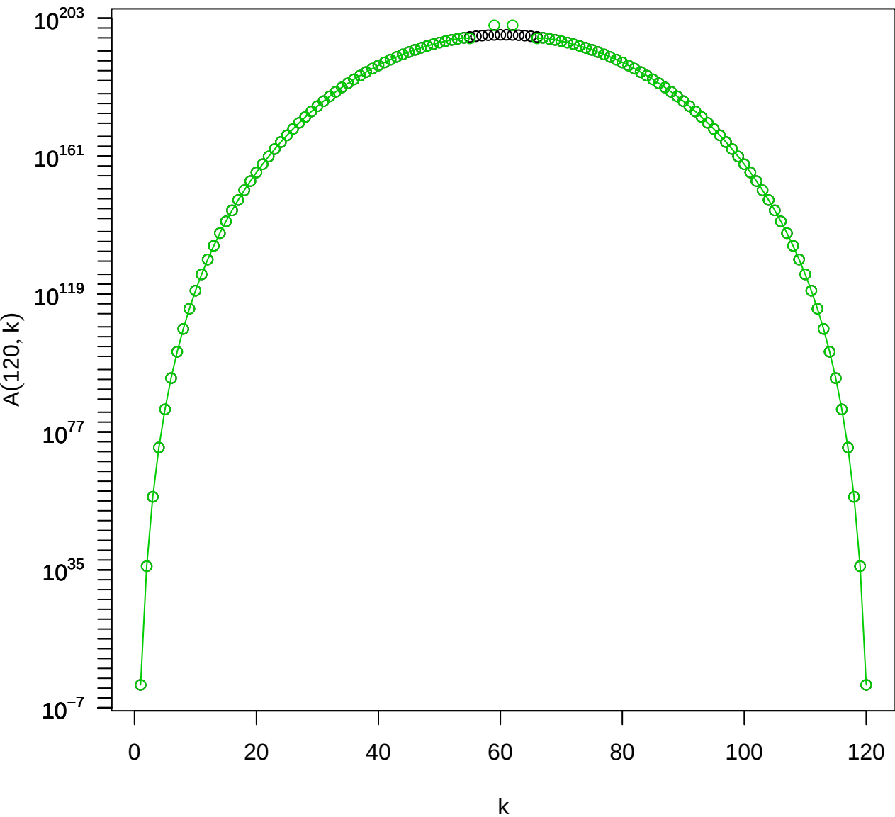
Eulerian numbers A(120, k)
