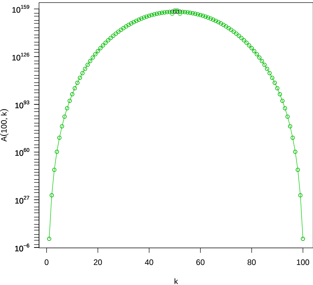
Eulerian numbers A(100, k)
