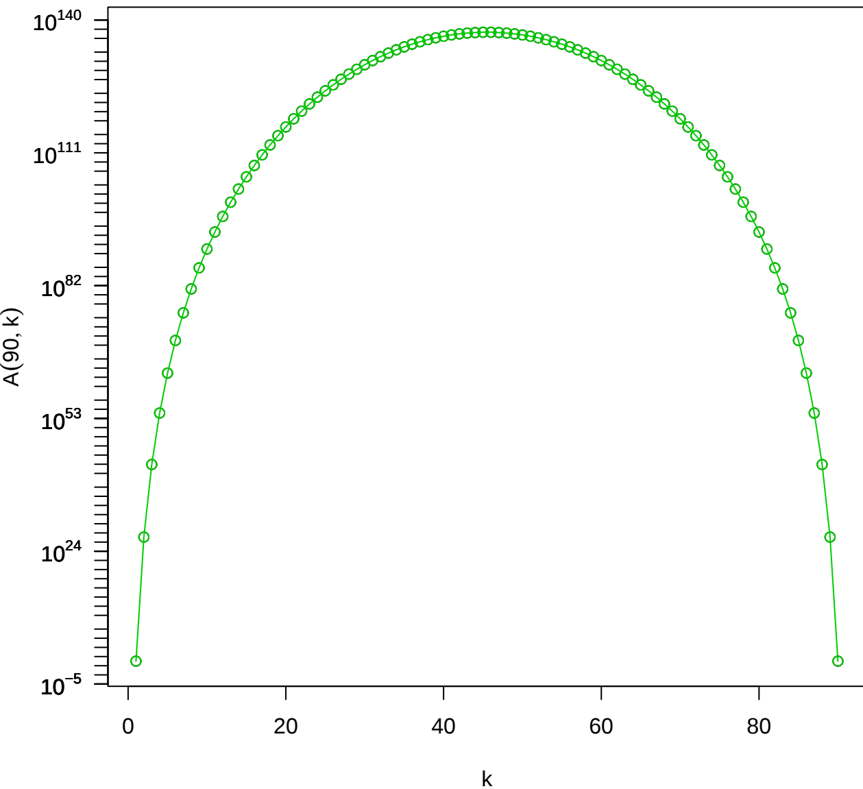
Eulerian numbers A(90, k)
