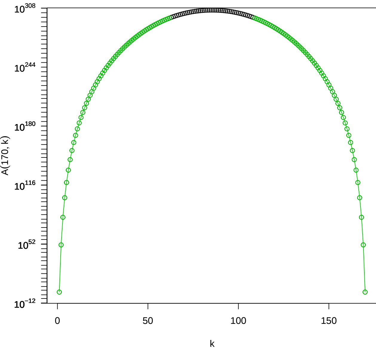
Eulerian numbers A(170, k)
