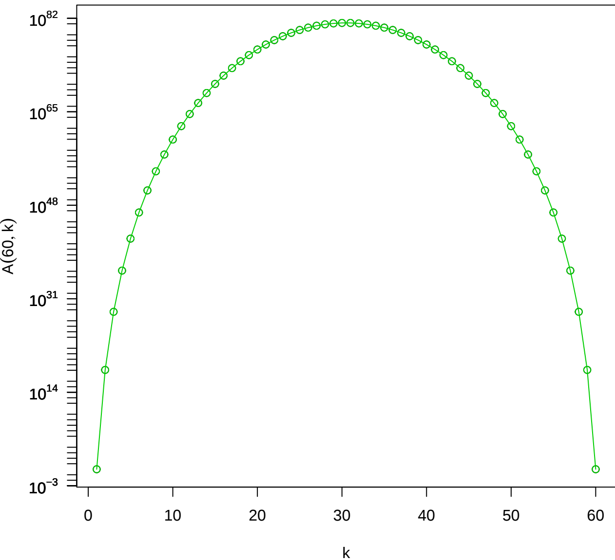
Eulerian numbers A(60, k)
