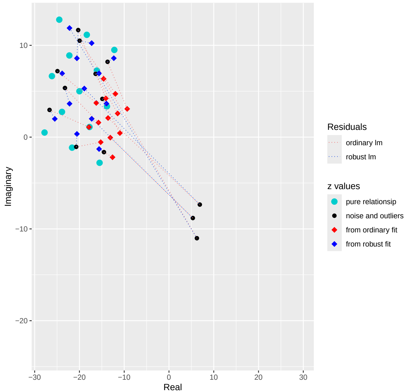
Generated and Fit Values of z
