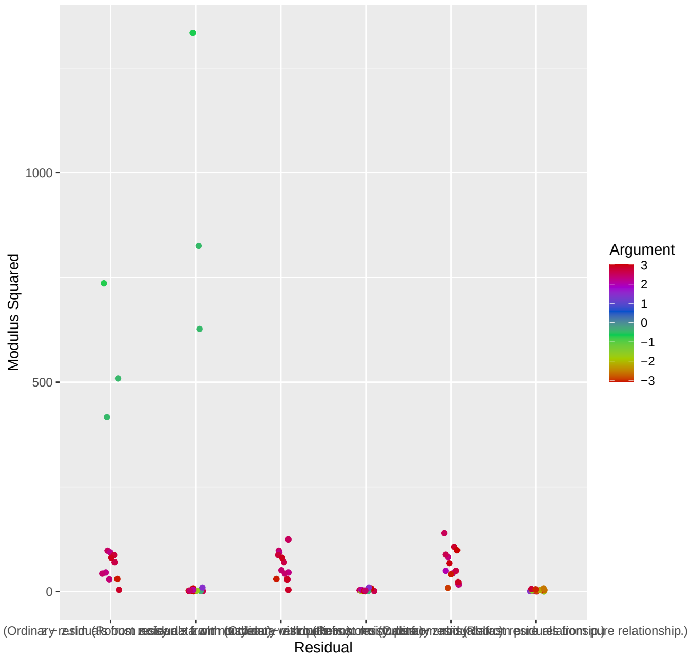
Squared Modulus of Residuals
